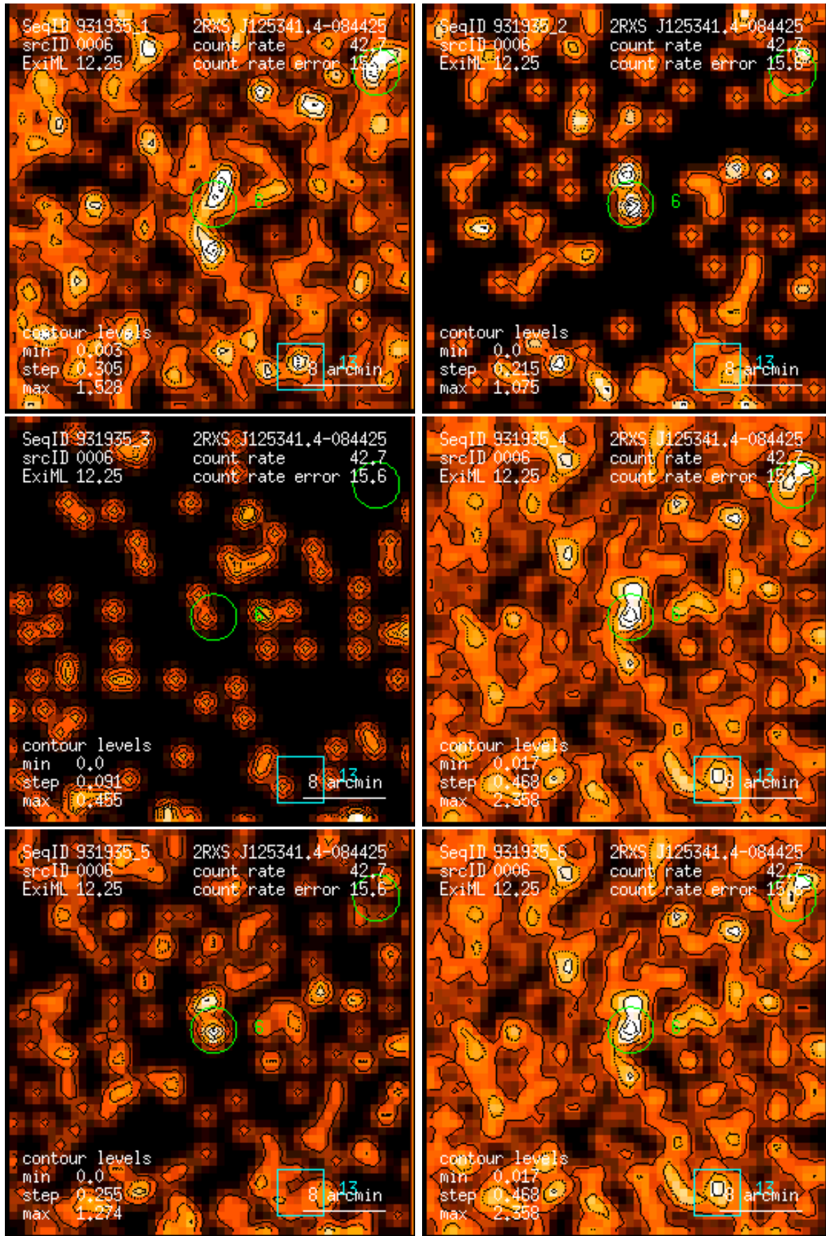
Figure 6: RASS 931935: detection 0006: band rate images, Gaussian filter: (1) PSPC channels 11 – 41, (2) 52 – 90, (3) 91 – 201, (4) 11 – 235, (5) 52 – 201, (6) 11 – 201. Broad band rates in counts/ks. Band rate contour levels in counts/ks/arcmin 2 .
