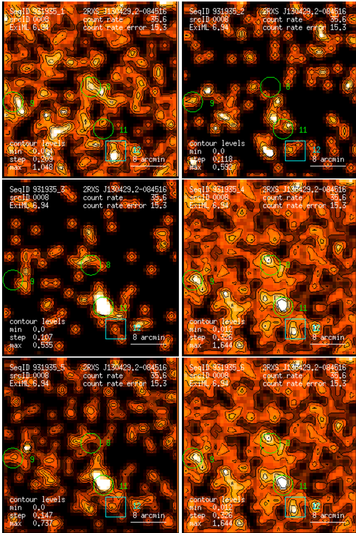
Figure 8: RASS 931935: detection 0008: band rate images, Gaussian filter: (1) PSPC channels 11 – 41, (2) 52 – 90, (3) 91 – 201, (4) 11 – 235, (5) 52 – 201, (6) 11 – 201. Broad band rates in counts/ks. Band rate contour levels in counts/ks/arcmin 2 .
