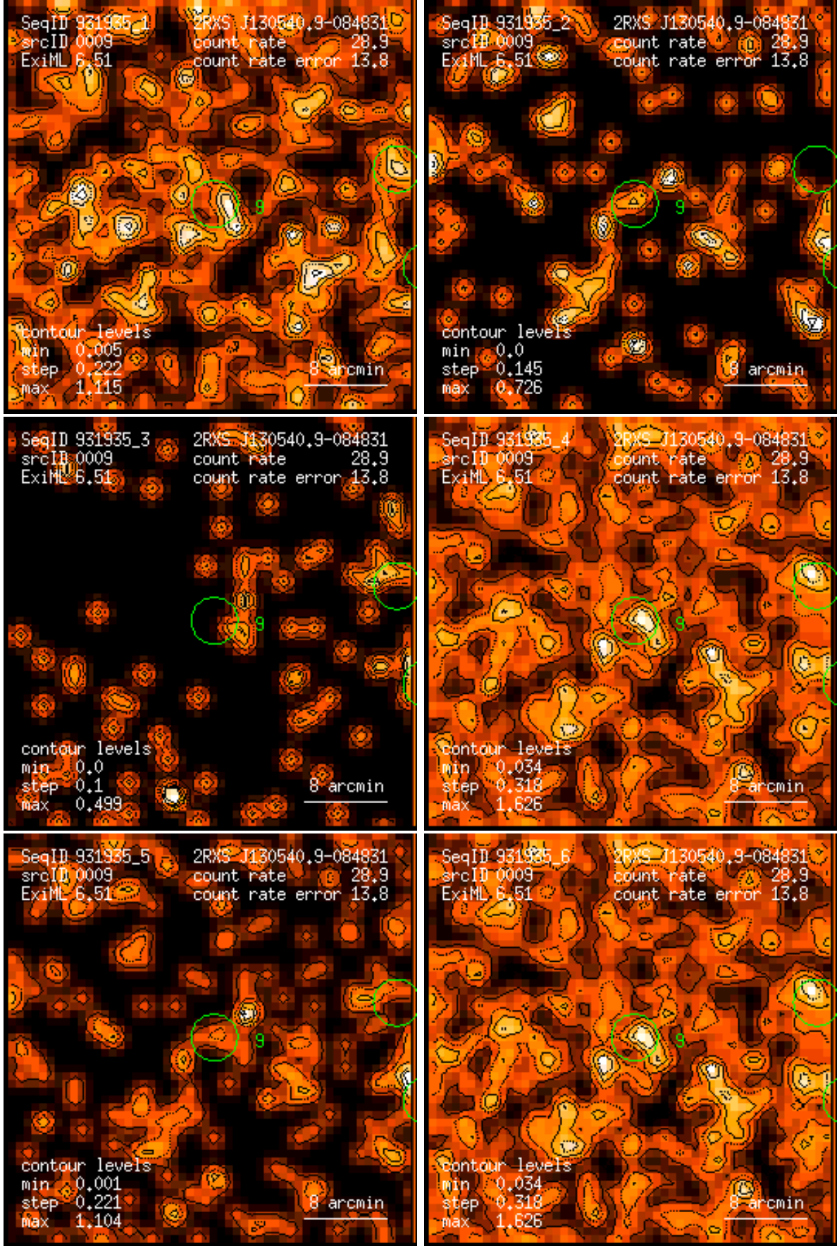
Figure 9: RASS 931935: detection 0009: band rate images, Gaussian filter: (1) PSPC channels 11 – 41, (2) 52 – 90, (3) 91 – 201, (4) 11 – 235, (5) 52 – 201, (6) 11 – 201. Broad band rates in counts/ks. Band rate contour levels in counts/ks/arcmin 2 .
