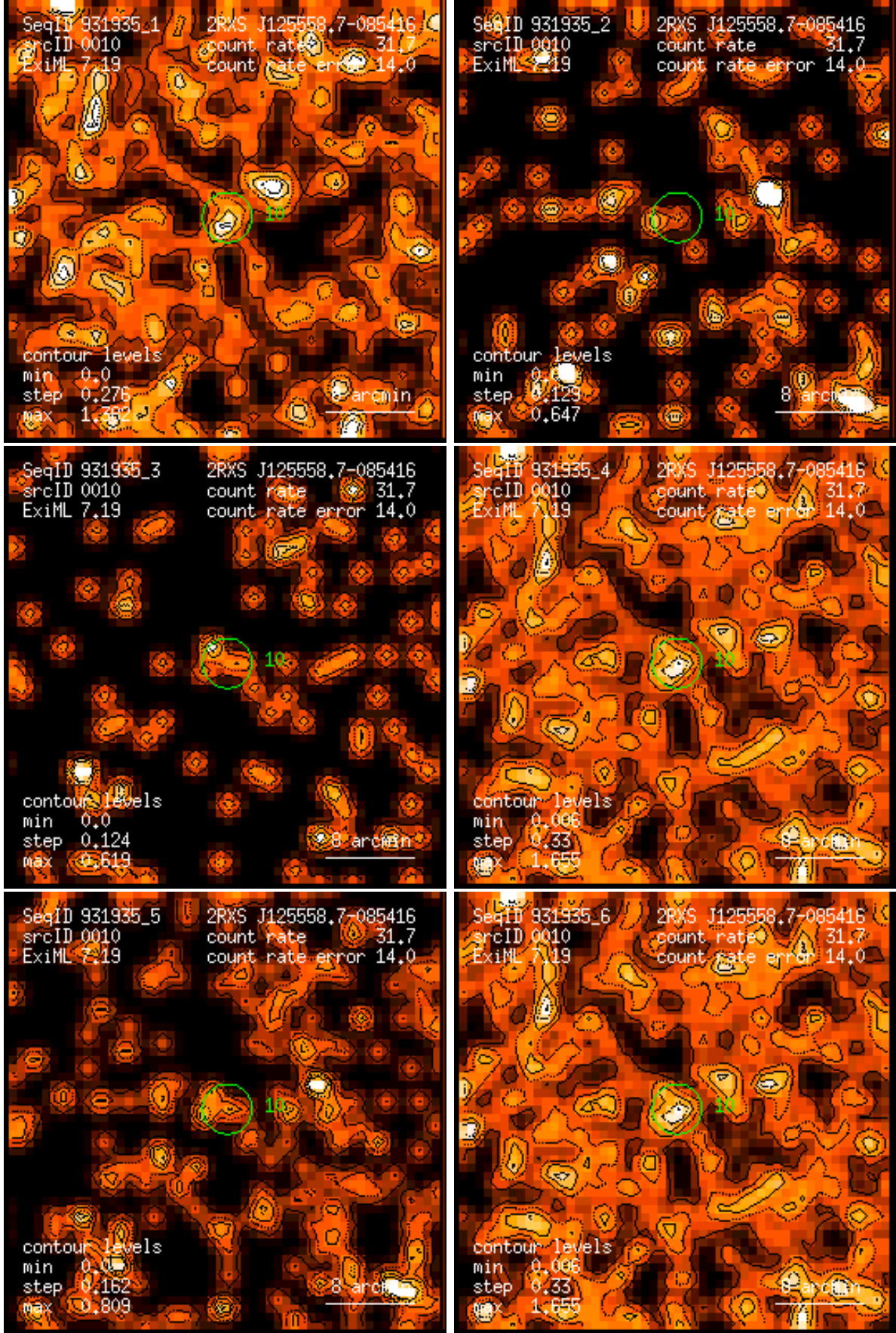
Figure 10: RASS 931935: detection 0010: band rate images, Gaussian filter: (1) PSPC channels 11 – 41, (2) 52 – 90, (3) 91 – 201, (4) 11 – 235, (5) 52 – 201, (6) 11 – 201. Broad band rates in counts/ks. Band rate contour levels in counts/ks/arcmin 2 .
