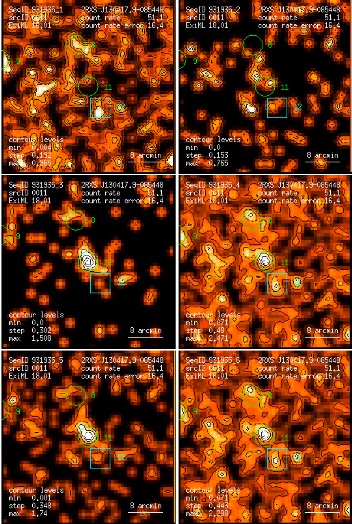
Figure 11: RASS 931935: detection 0011: band rate images, Gaussian filter: (1) PSPC channels 11 – 41, (2) 52 – 90, (3) 91 – 201, (4) 11 – 235, (5) 52 – 201, (6) 11 – 201. Broad band rates in counts/ks. Band rate contour levels in counts/ks/arcmin 2 .
