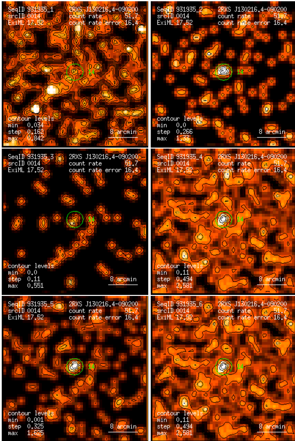
Figure 14: RASS 931935: detection 0014: band rate images, Gaussian filter: (1) PSPC channels 11 – 41, (2) 52 – 90, (3) 91 – 201, (4) 11 – 235, (5) 52 – 201, (6) 11 – 201. Broad band rates in counts/ks. Band rate contour levels in counts/ks/arcmin 2 .
