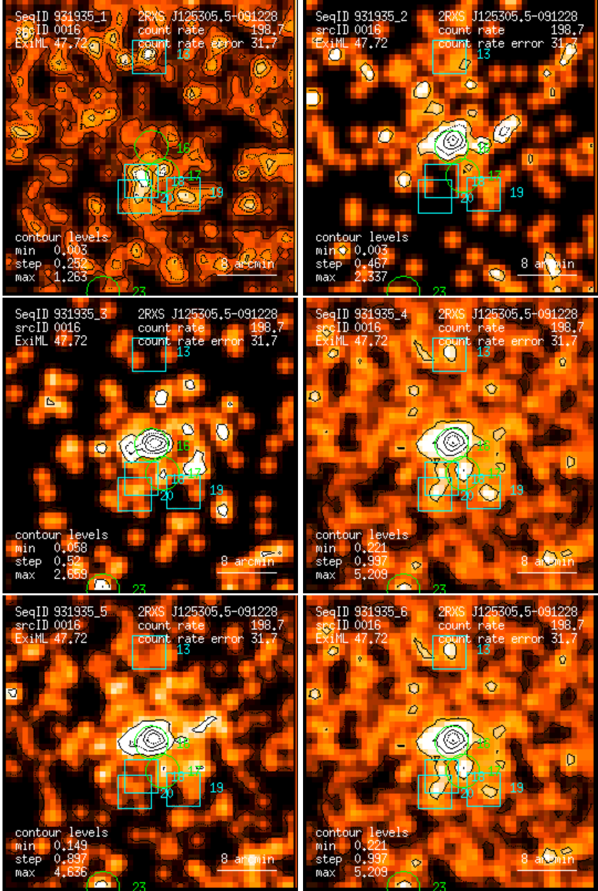
Figure 16: RASS 931935: detection 0016: band rate images, Gaussian filter: (1) PSPC channels 11 – 41, (2) 52 – 90, (3) 91 – 201, (4) 11 – 235, (5) 52 – 201, (6) 11 – 201. Broad band rates in counts/ks. Band rate contour levels in counts/ks/arcmin 2 .
