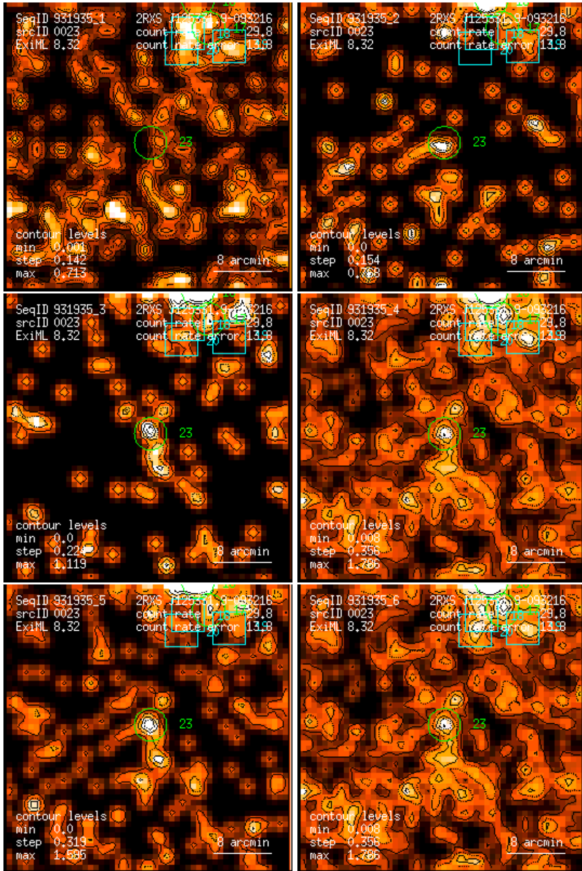
Figure 23: RASS 931935: detection 0023: band rate images, Gaussian filter: (1) PSPC channels 11 – 41, (2) 52 – 90, (3) 91 – 201, (4) 11 – 235, (5) 52 – 201, (6) 11 – 201. Broad band rates in counts/ks. Band rate contour levels in counts/ks/arcmin 2 .
