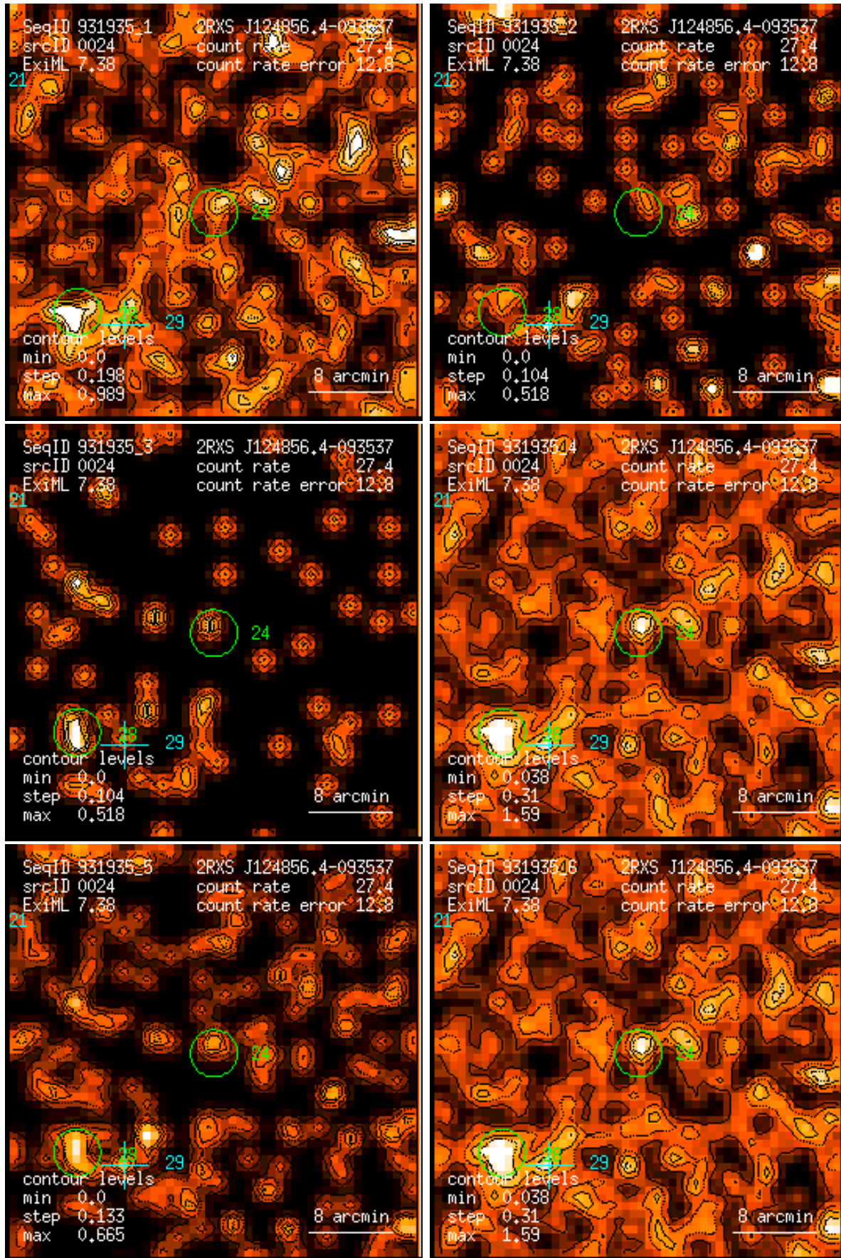
Figure 24: RASS 931935: detection 0024: band rate images, Gaussian filter: (1) PSPC channels 11 – 41, (2) 52 – 90, (3) 91 – 201, (4) 11 – 235, (5) 52 – 201, (6) 11 – 201. Broad band rates in counts/ks. Band rate contour levels in counts/ks/arcmin 2 .
