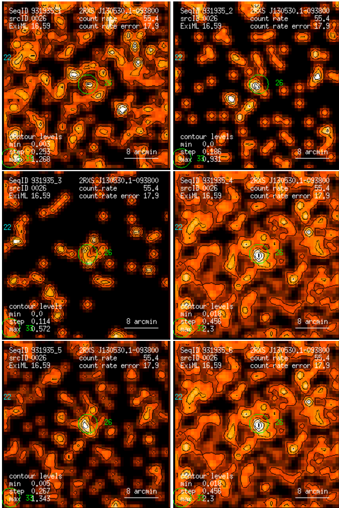
Figure 26: RASS 931935: detection 0026: band rate images, Gaussian filter: (1) PSPC channels 11 – 41, (2) 52 – 90, (3) 91 – 201, (4) 11 – 235, (5) 52 – 201, (6) 11 – 201. Broad band rates in counts/ks. Band rate contour levels in counts/ks/arcmin 2 .
