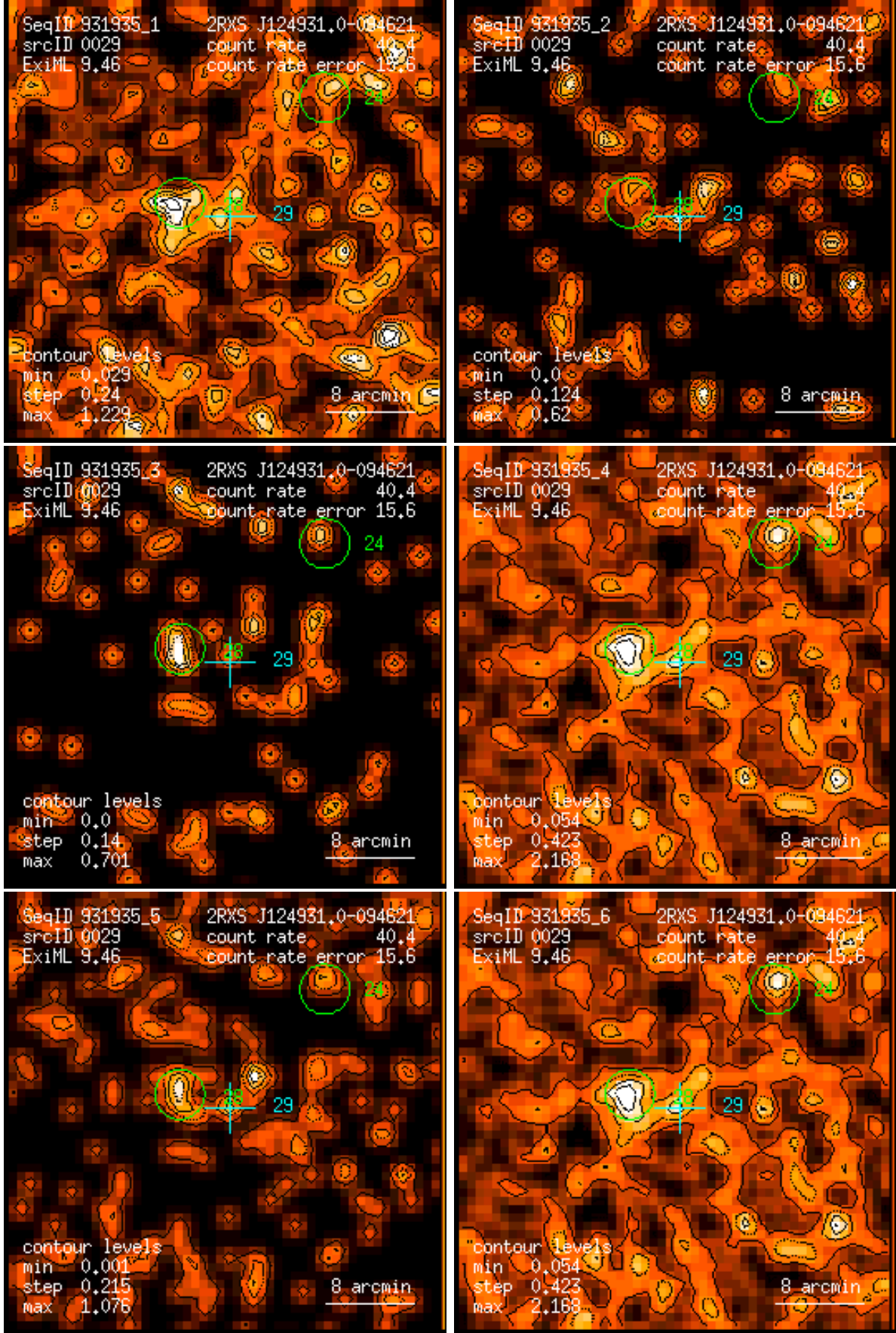
Figure 29: RASS 931935: detection 0029: band rate images, Gaussian filter: (1) PSPC channels 11 – 41, (2) 52 – 90, (3) 91 – 201, (4) 11 – 235, (5) 52 – 201, (6) 11 – 201. Broad band rates in counts/ks. Band rate contour levels in counts/ks/arcmin 2 .
