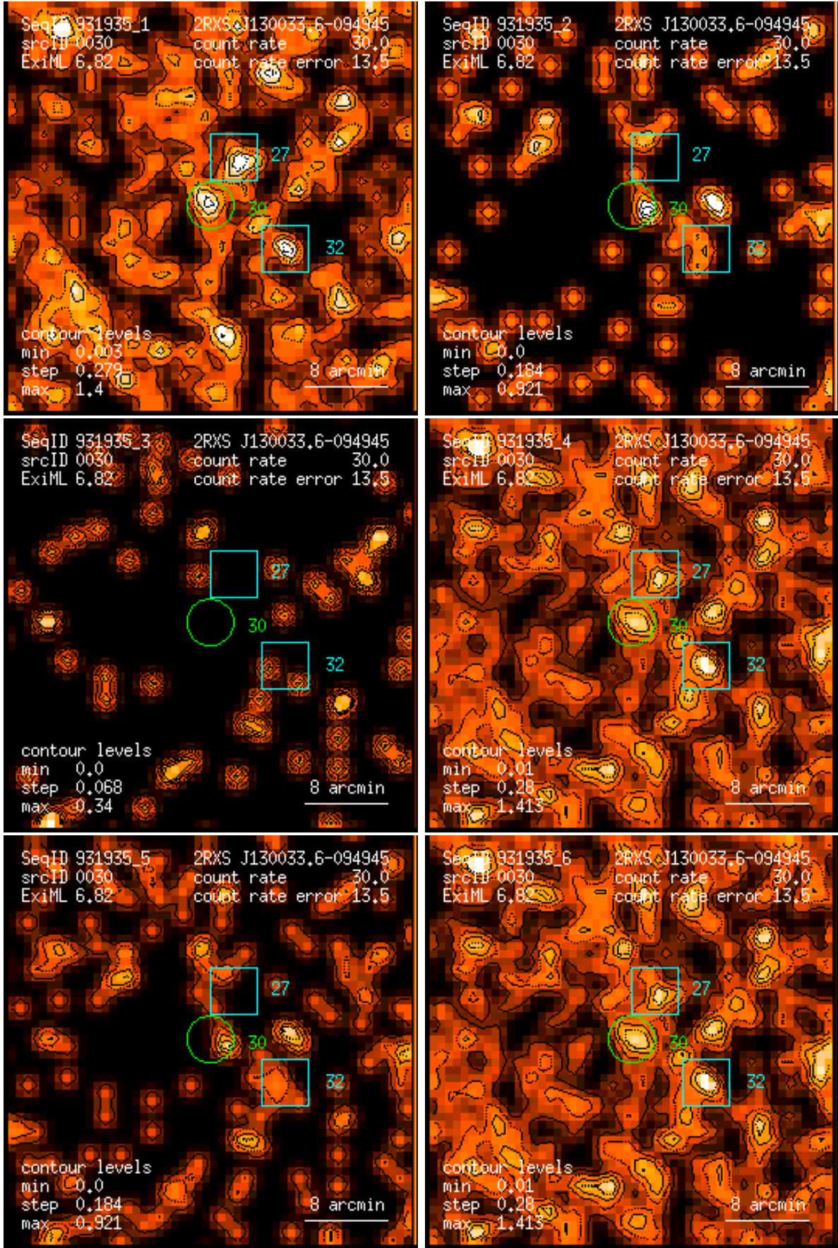
Figure 30: RASS 931935: detection 0030: band rate images, Gaussian filter: (1) PSPC channels 11 – 41, (2) 52 – 90, (3) 91 – 201, (4) 11 – 235, (5) 52 – 201, (6) 11 – 201. Broad band rates in counts/ks. Band rate contour levels in counts/ks/arcmin 2 .
