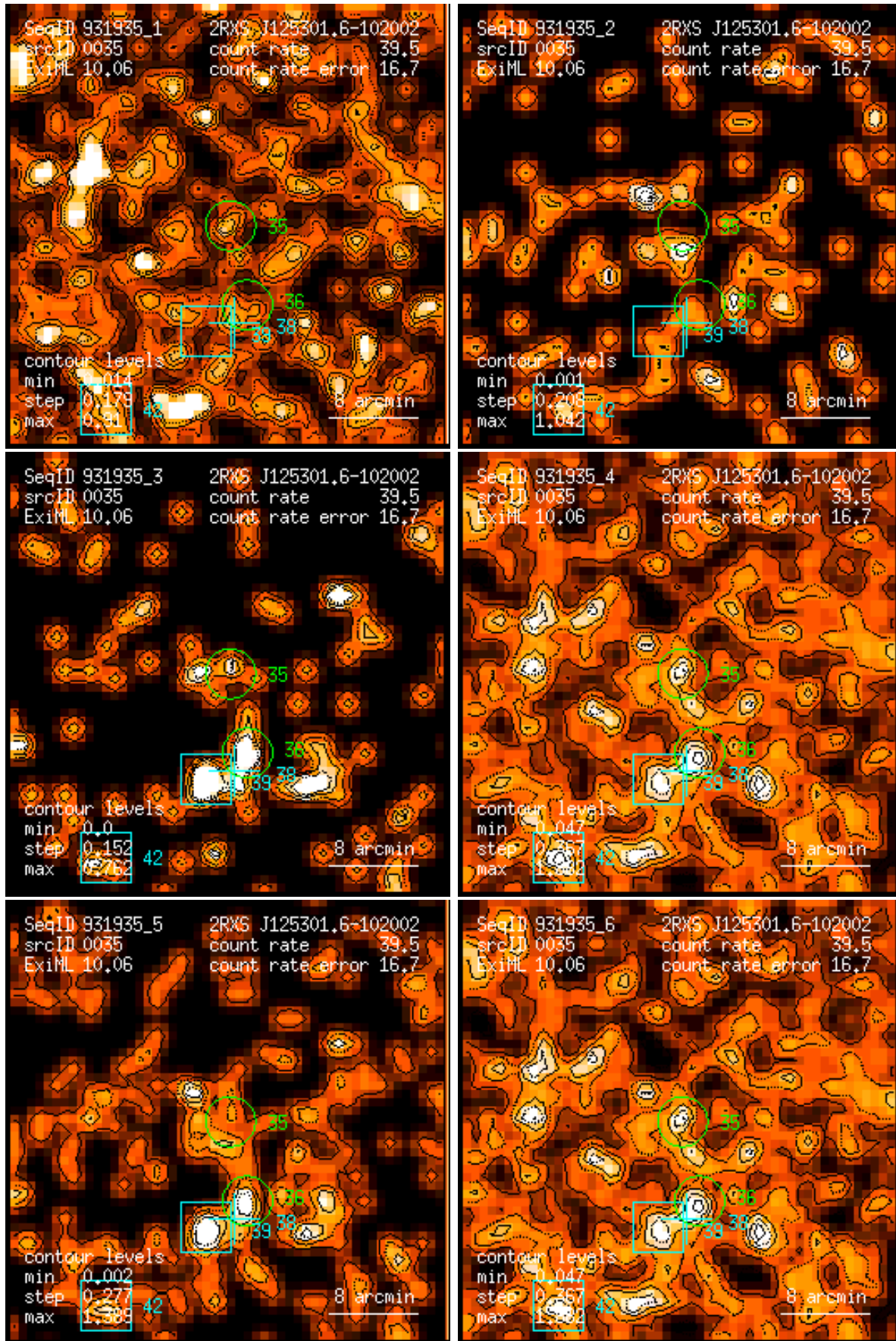
Figure 35: RASS 931935: detection 0035: band rate images, Gaussian filter: (1) PSPC channels 11 – 41, (2) 52 – 90, (3) 91 – 201, (4) 11 – 235, (5) 52 – 201, (6) 11 – 201. Broad band rates in counts/ks. Band rate contour levels in counts/ks/arcmin 2 .
