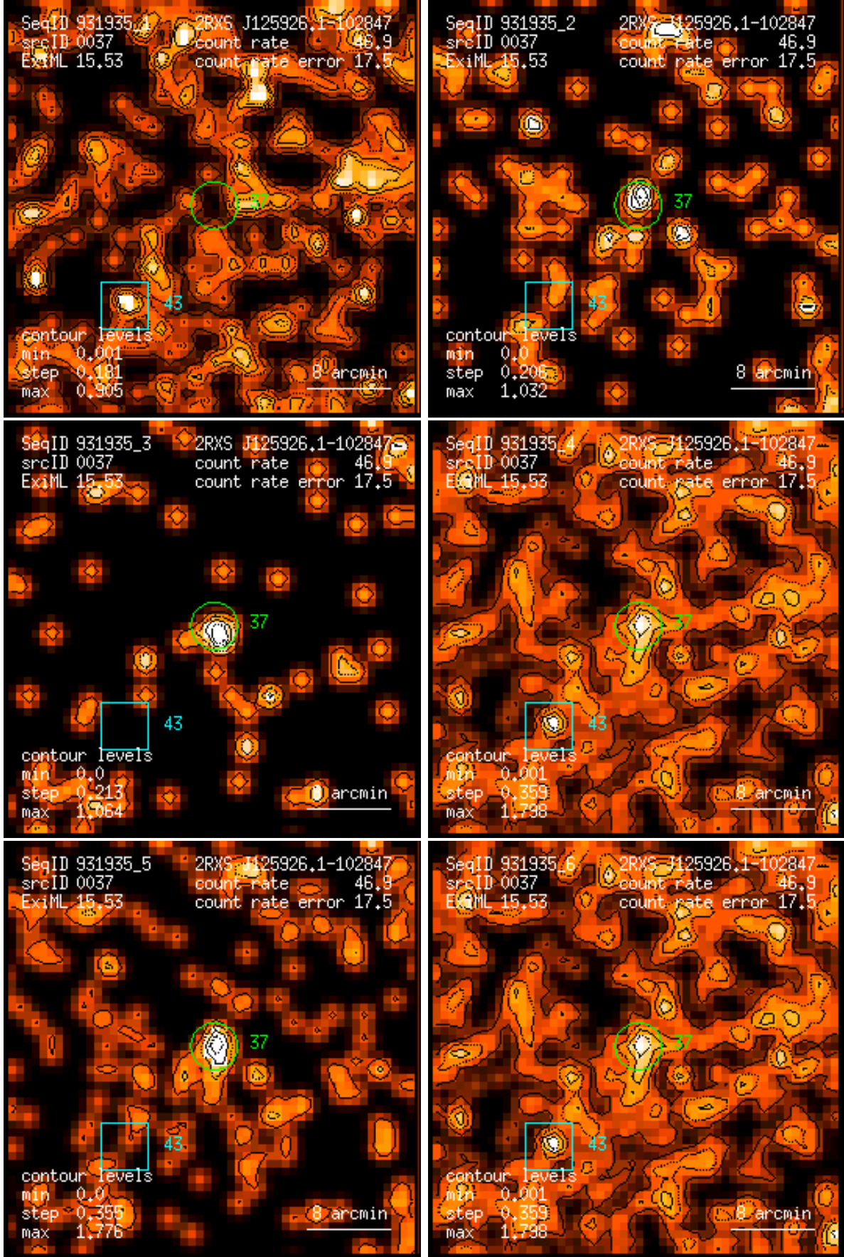
Figure 37: RASS 931935: detection 0037: band rate images, Gaussian filter: (1) PSPC channels 11 – 41, (2) 52 – 90, (3) 91 – 201, (4) 11 – 235, (5) 52 – 201, (6) 11 – 201. Broad band rates in counts/ks. Band rate contour levels in counts/ks/arcmin 2 .
