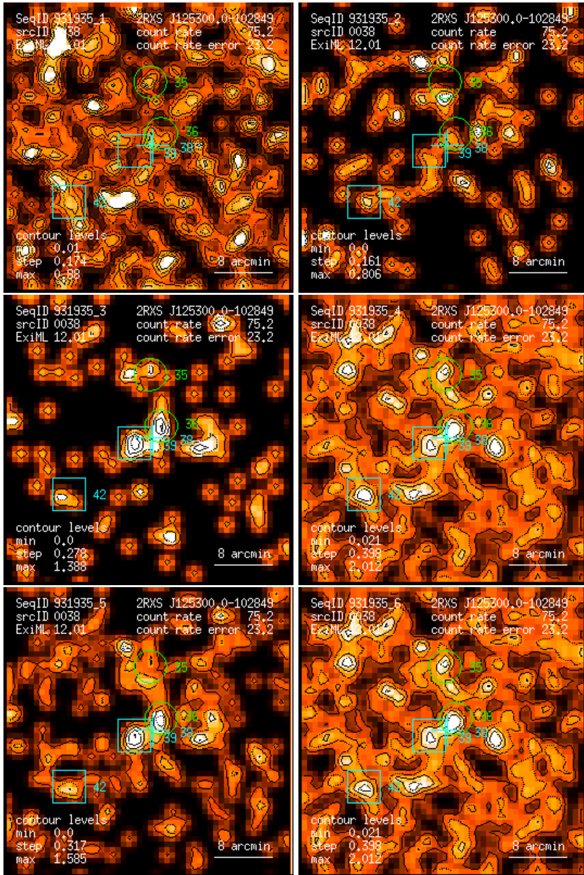
Figure 38: RASS 931935: detection 0038: band rate images, Gaussian filter: (1) PSPC channels 11 – 41, (2) 52 – 90, (3) 91 – 201, (4) 11 – 235, (5) 52 – 201, (6) 11 – 201. Broad band rates in counts/ks. Band rate contour levels in counts/ks/arcmin 2 .
