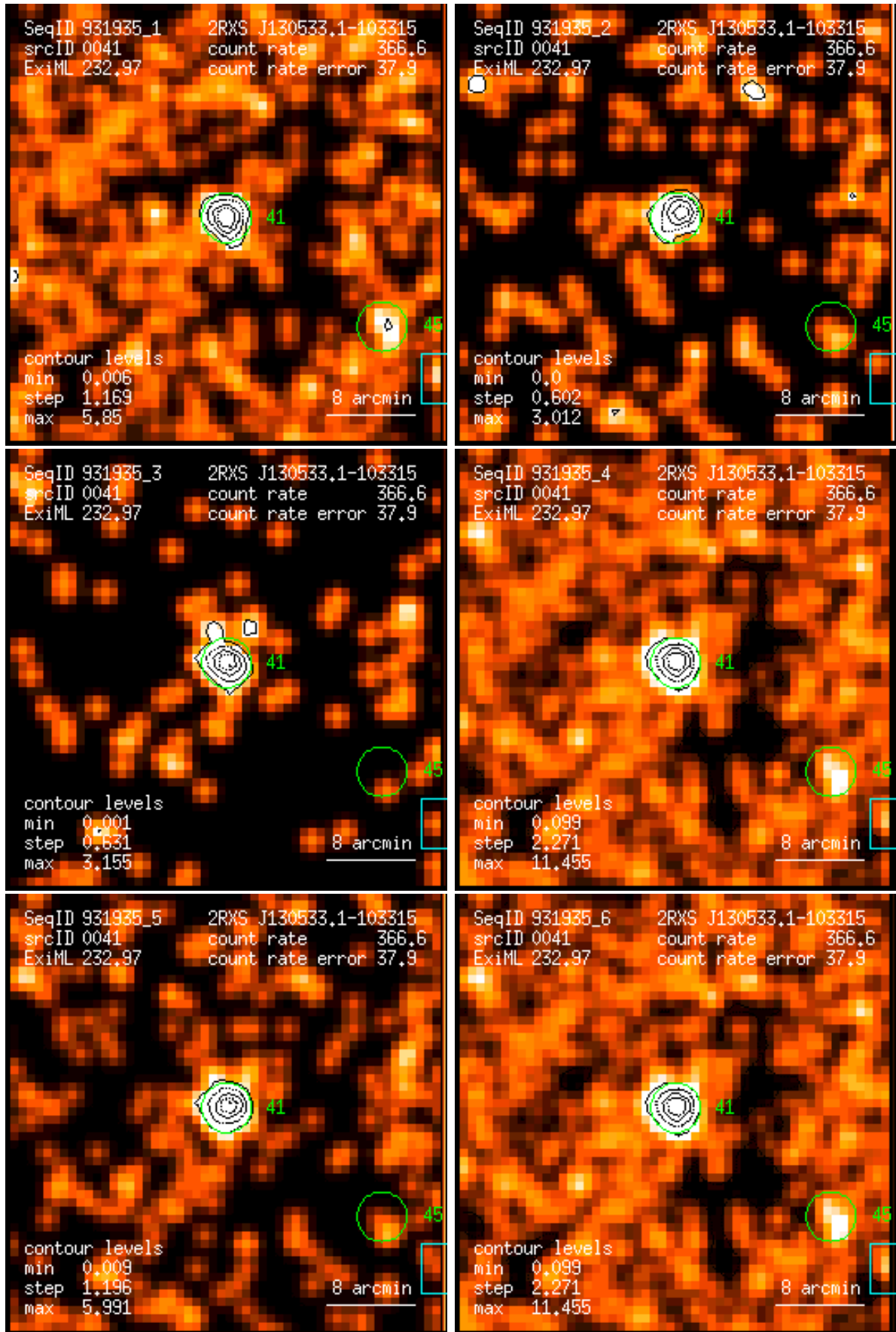
Figure 41: RASS 931935: detection 0041: band rate images, Gaussian filter: (1) PSPC channels 11 – 41, (2) 52 – 90, (3) 91 – 201, (4) 11 – 235, (5) 52 – 201, (6) 11 – 201. Broad band rates in counts/ks. Band rate contour levels in counts/ks/arcmin 2 .
