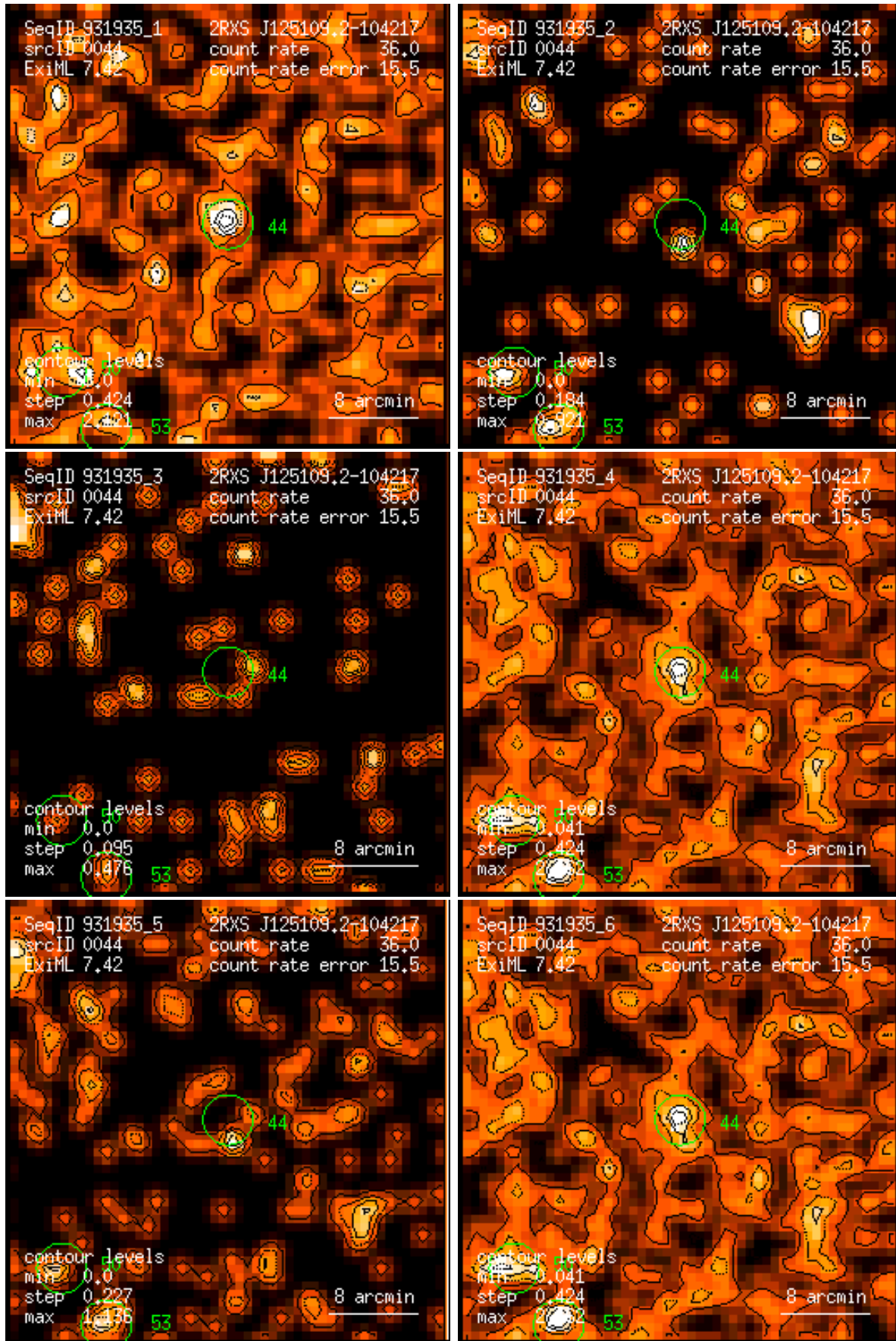
Figure 44: RASS 931935: detection 0044: band rate images, Gaussian filter: (1) PSPC channels 11 – 41, (2) 52 – 90, (3) 91 – 201, (4) 11 – 235, (5) 52 – 201, (6) 11 – 201. Broad band rates in counts/ks. Band rate contour levels in counts/ks/arcmin 2 .
