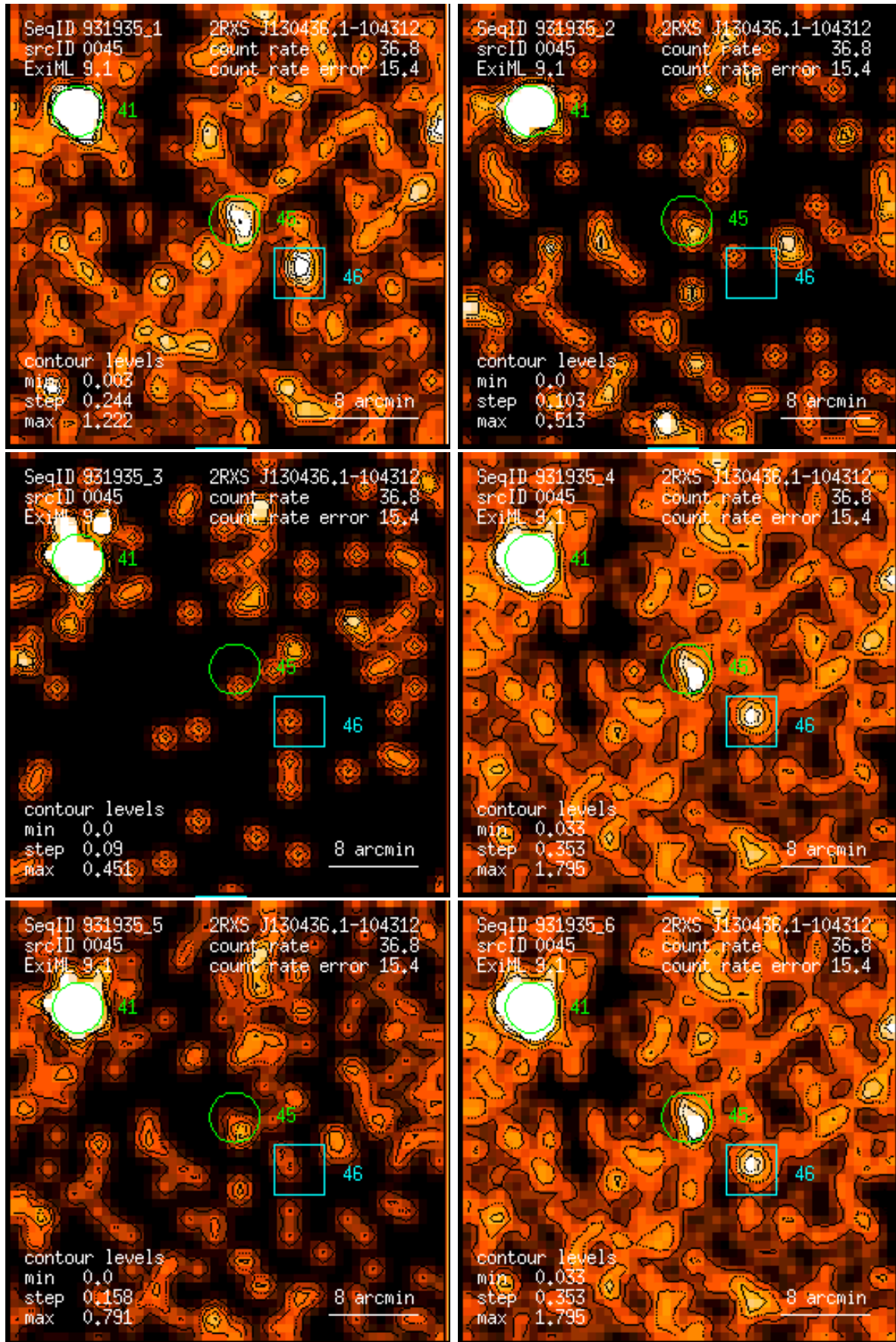
Figure 45: RASS 931935: detection 0045: band rate images, Gaussian filter: (1) PSPC channels 11 – 41, (2) 52 – 90, (3) 91 – 201, (4) 11 – 235, (5) 52 – 201, (6) 11 – 201. Broad band rates in counts/ks. Band rate contour levels in counts/ks/arcmin 2 .
