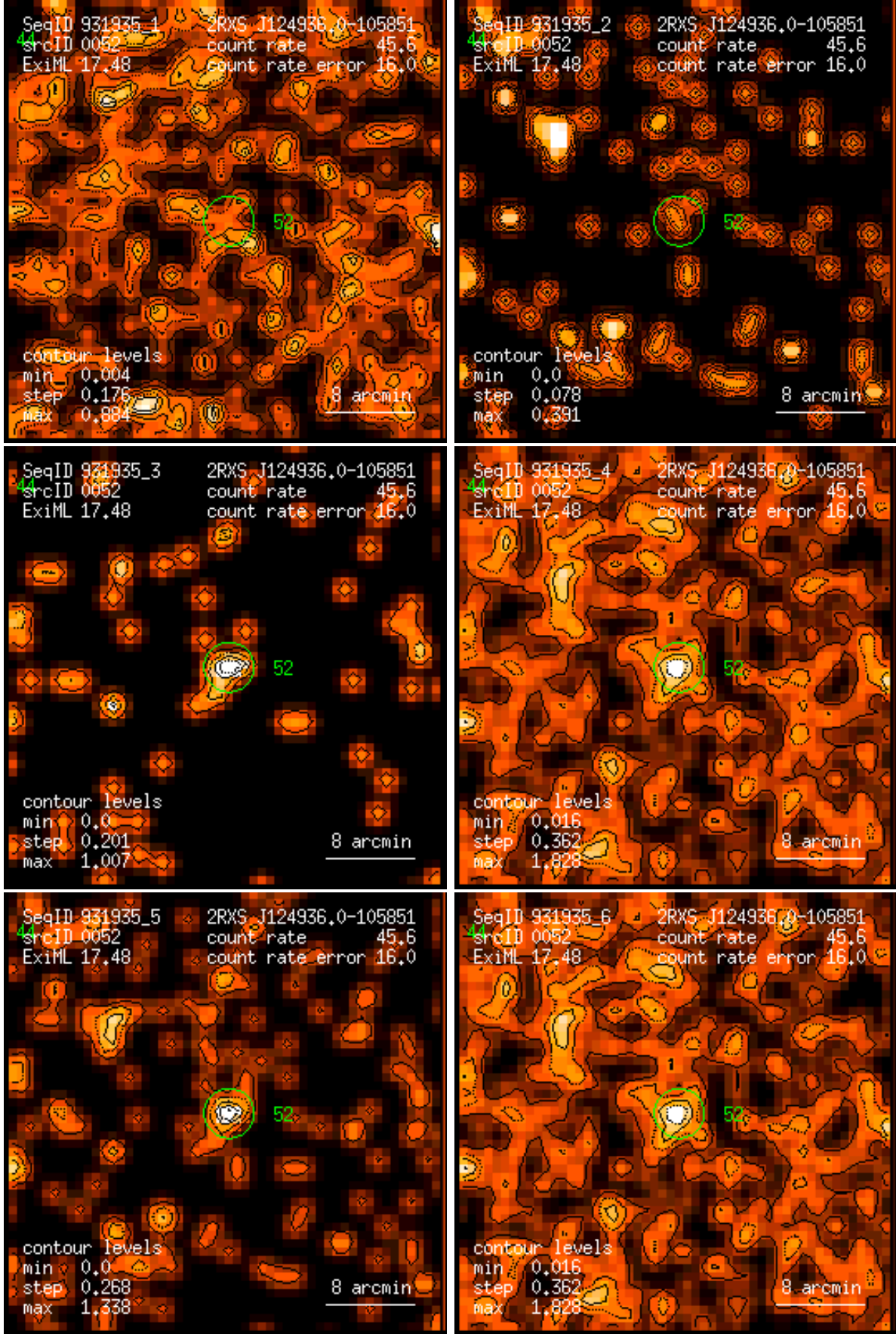
Figure 52: RASS 931935: detection 0052: band rate images, Gaussian filter: (1) PSPC channels 11 – 41, (2) 52 – 90, (3) 91 – 201, (4) 11 – 235, (5) 52 – 201, (6) 11 – 201. Broad band rates in counts/ks. Band rate contour levels in counts/ks/arcmin 2 .
