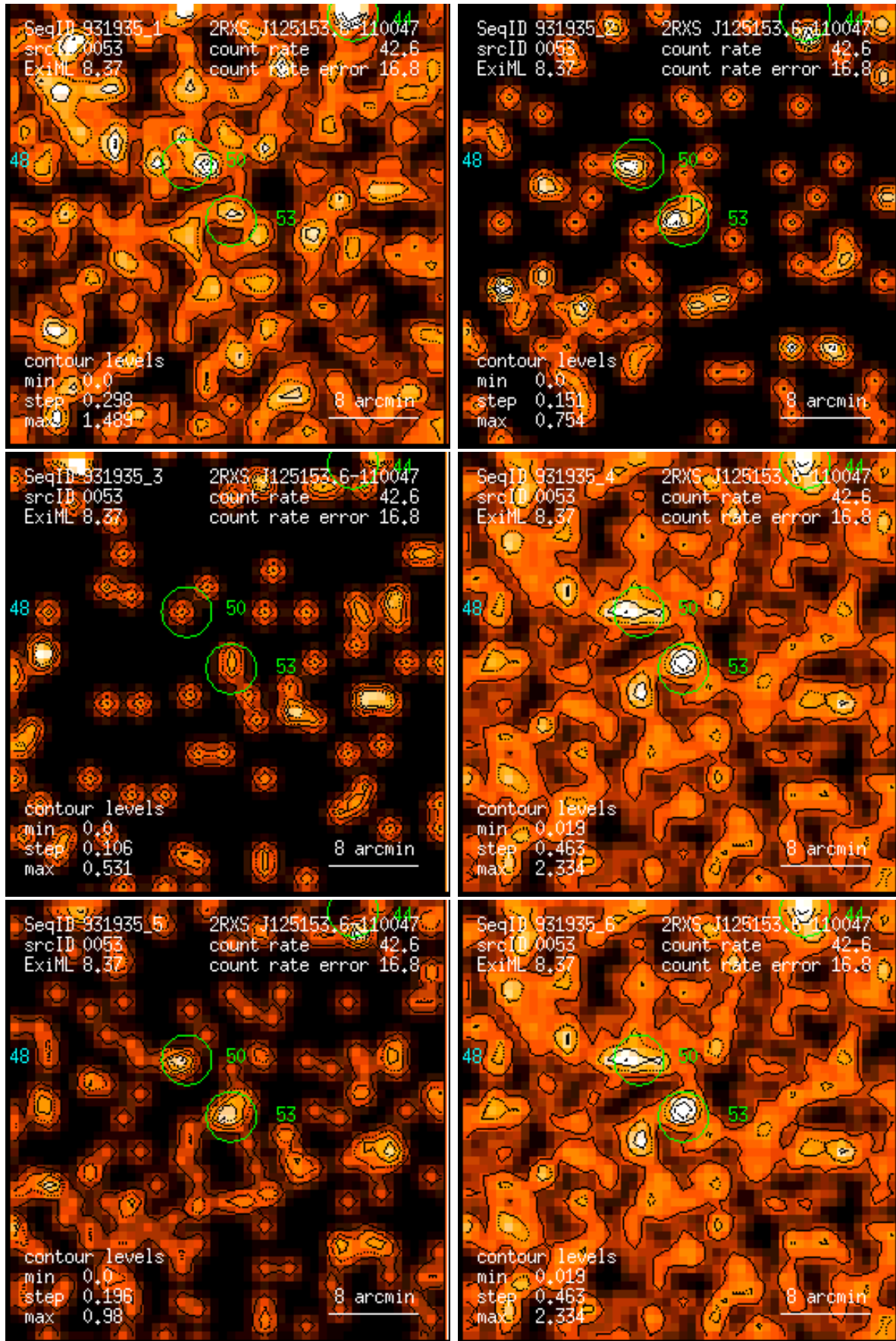
Figure 53: RASS 931935: detection 0053: band rate images, Gaussian filter: (1) PSPC channels 11 – 41, (2) 52 – 90, (3) 91 – 201, (4) 11 – 235, (5) 52 – 201, (6) 11 – 201. Broad band rates in counts/ks. Band rate contour levels in counts/ks/arcmin 2 .
