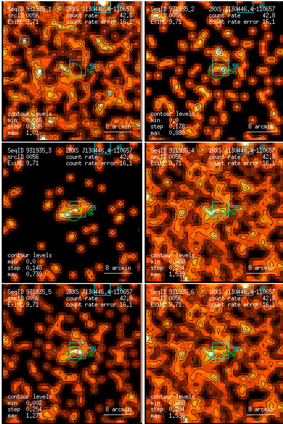
Figure 56: RASS 931935: detection 0056: band rate images, Gaussian filter: (1) PSPC channels 11 – 41, (2) 52 – 90, (3) 91 – 201, (4) 11 – 235, (5) 52 – 201, (6) 11 – 201. Broad band rates in counts/ks. Band rate contour levels in counts/ks/arcmin 2 .
