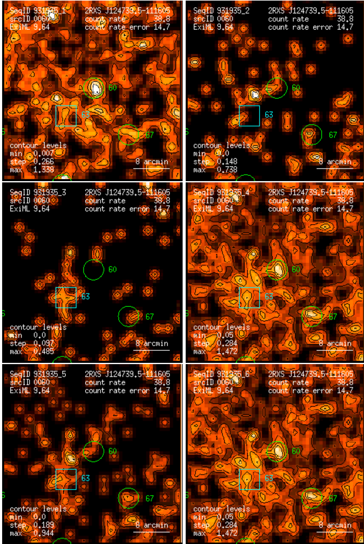
Figure 60: RASS 931935: detection 0060: band rate images, Gaussian filter: (1) PSPC channels 11 – 41, (2) 52 – 90, (3) 91 – 201, (4) 11 – 235, (5) 52 – 201, (6) 11 – 201. Broad band rates in counts/ks. Band rate contour levels in counts/ks/arcmin 2 .
