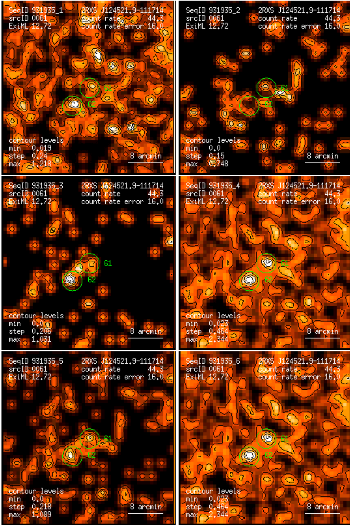
Figure 61: RASS 931935: detection 0061: band rate images, Gaussian filter: (1) PSPC channels 11 – 41, (2) 52 – 90, (3) 91 – 201, (4) 11 – 235, (5) 52 – 201, (6) 11 – 201. Broad band rates in counts/ks. Band rate contour levels in counts/ks/arcmin 2 .
