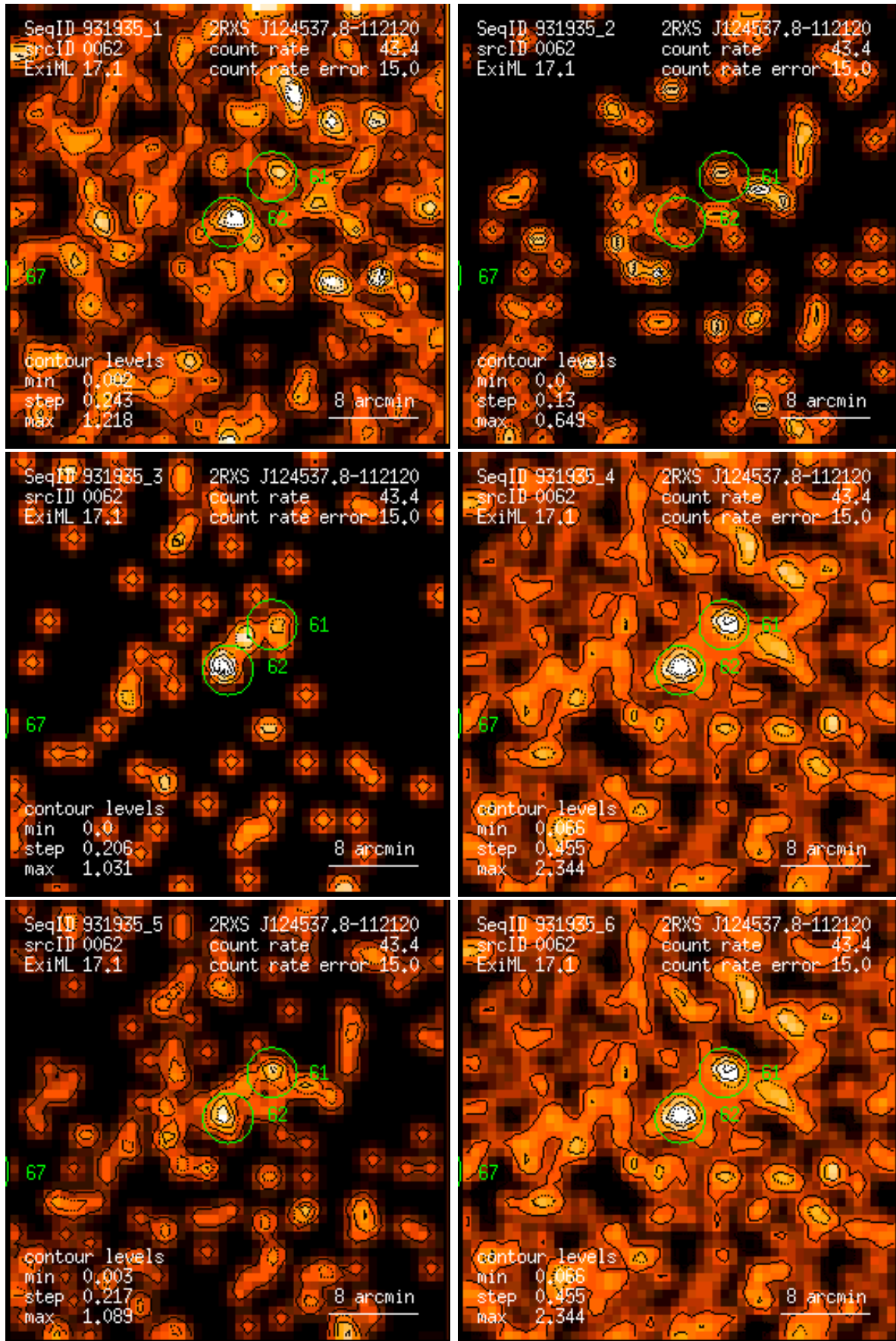
Figure 62: RASS 931935: detection 0062: band rate images, Gaussian filter: (1) PSPC channels 11 – 41, (2) 52 – 90, (3) 91 – 201, (4) 11 – 235, (5) 52 – 201, (6) 11 – 201. Broad band rates in counts/ks. Band rate contour levels in counts/ks/arcmin 2 .
