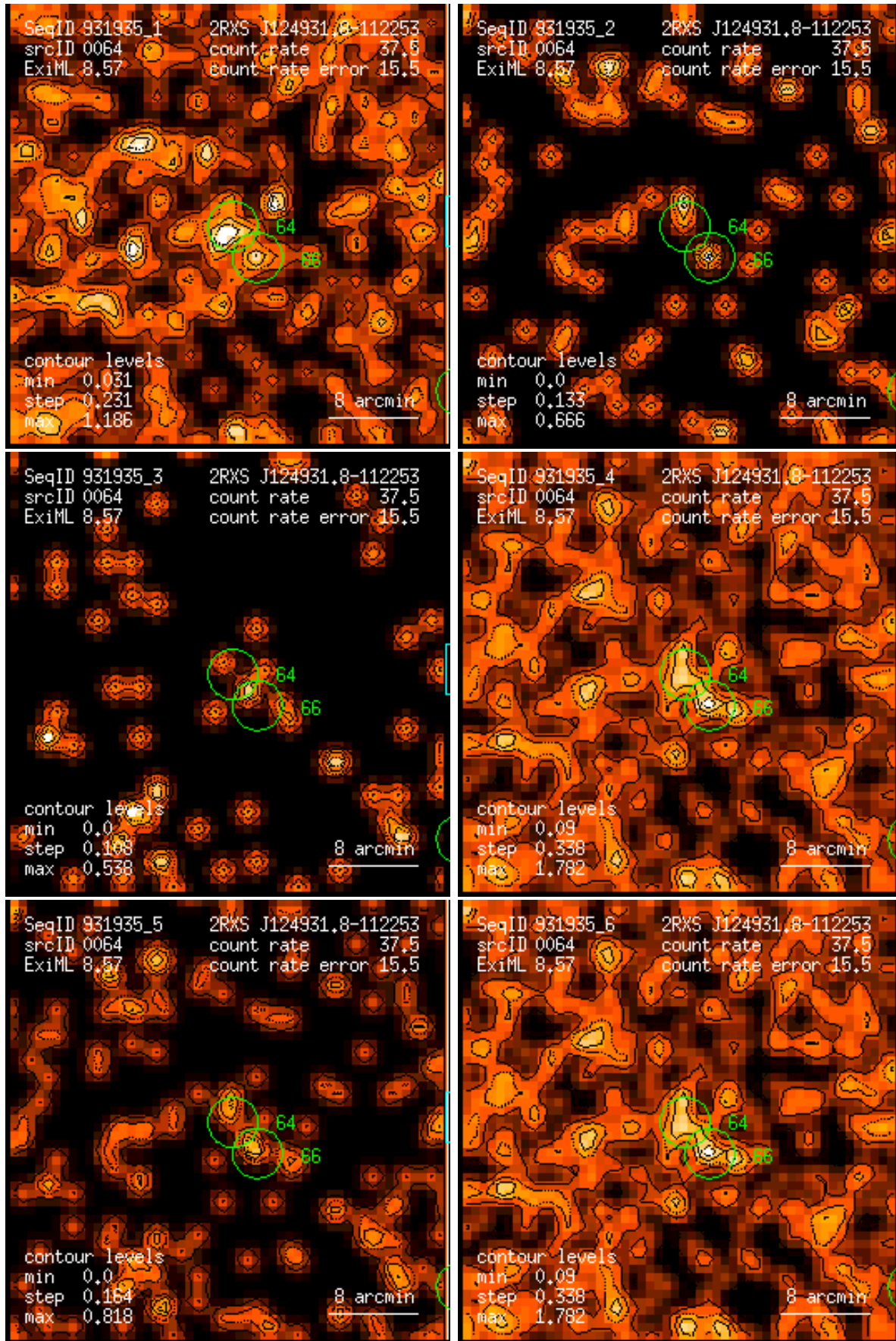
Figure 64: RASS 931935: detection 0064: band rate images, Gaussian filter: (1) PSPC channels 11 – 41, (2) 52 – 90, (3) 91 – 201, (4) 11 – 235, (5) 52 – 201, (6) 11 – 201. Broad band rates in counts/ks. Band rate contour levels in counts/ks/arcmin 2 .
