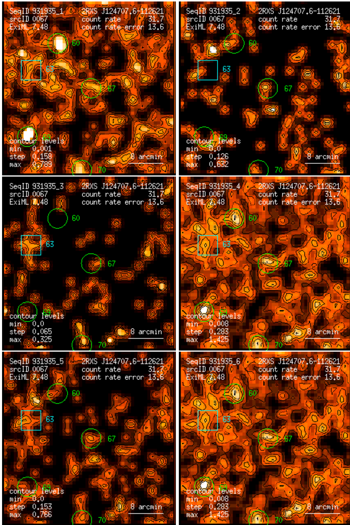
Figure 67: RASS 931935: detection 0067: band rate images, Gaussian filter: (1) PSPC channels 11 – 41, (2) 52 – 90, (3) 91 – 201, (4) 11 – 235, (5) 52 – 201, (6) 11 – 201. Broad band rates in counts/ks. Band rate contour levels in counts/ks/arcmin 2 .
