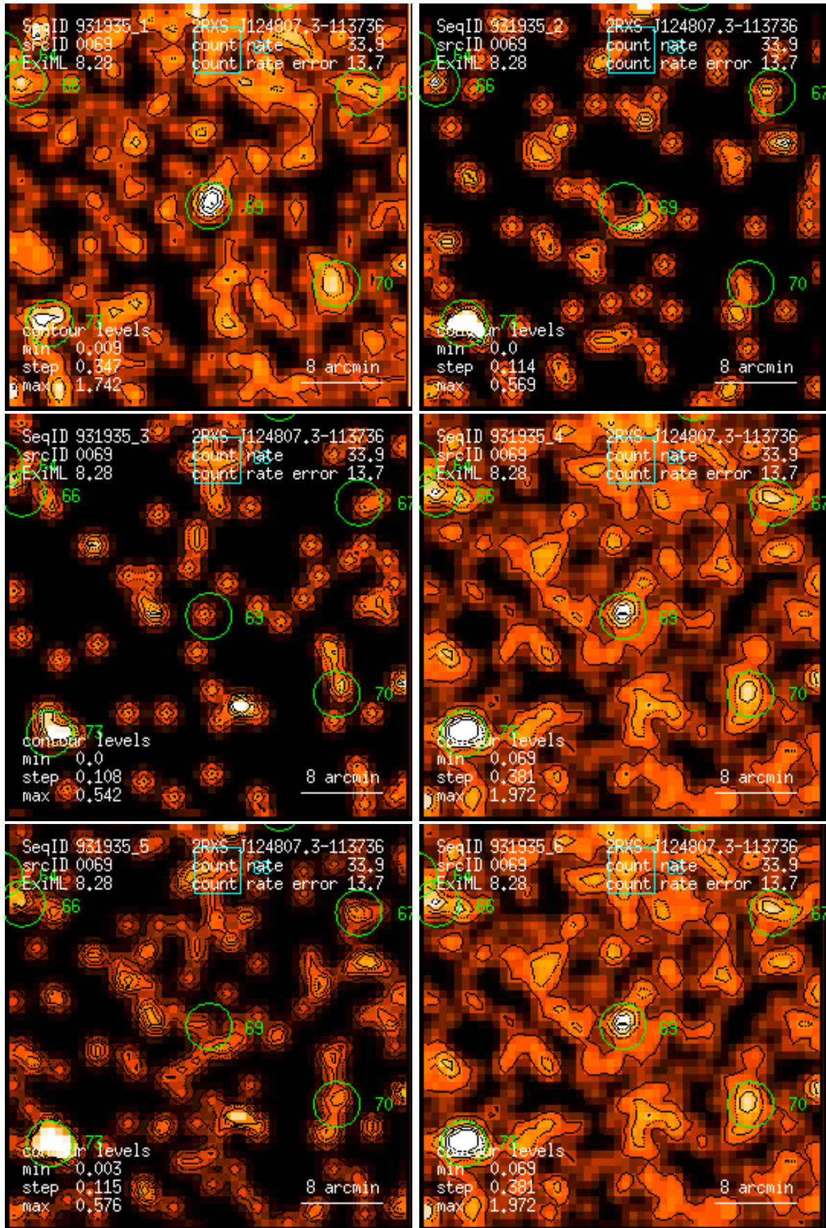
Figure 69: RASS 931935: detection 0069: band rate images, Gaussian filter: (1) PSPC channels 11 – 41, (2) 52 – 90, (3) 91 – 201, (4) 11 – 235, (5) 52 – 201, (6) 11 – 201. Broad band rates in counts/ks. Band rate contour levels in counts/ks/arcmin 2 .
