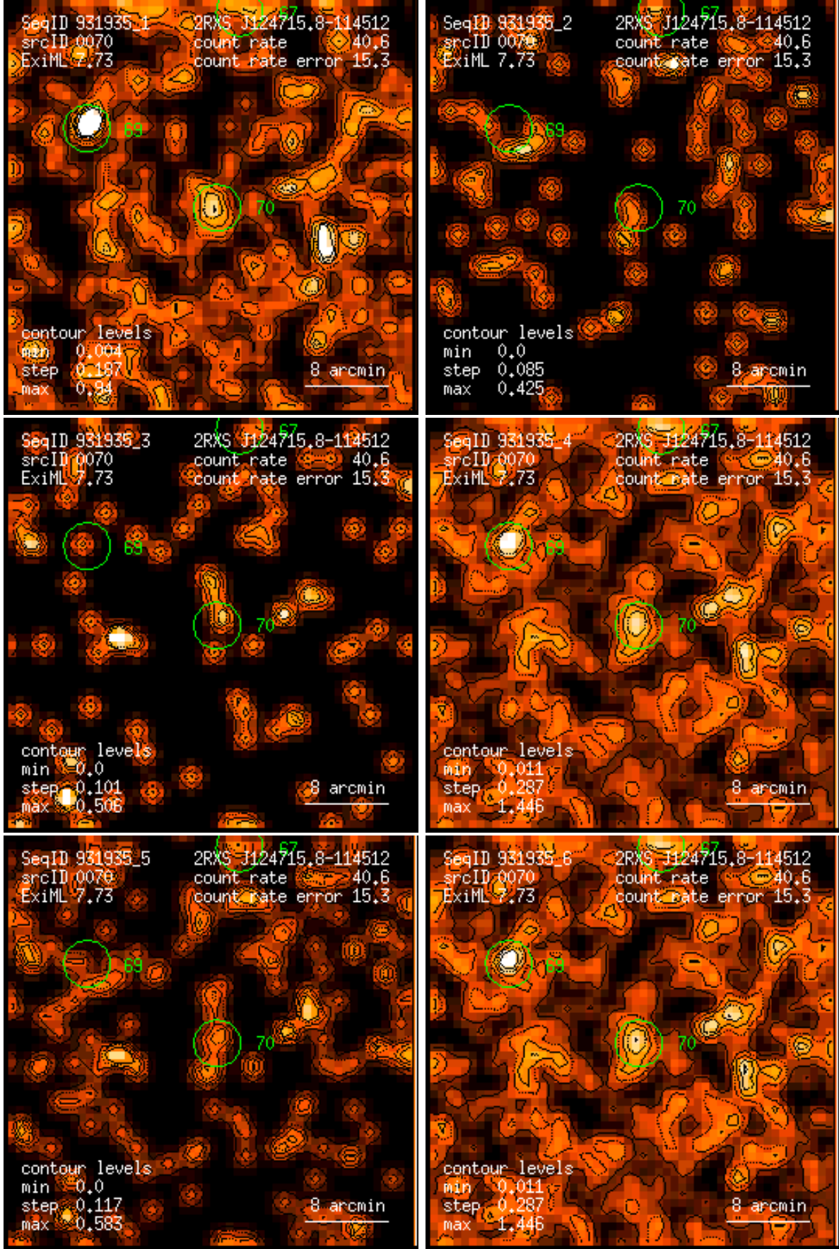
Figure 70: RASS 931935: detection 0070: band rate images, Gaussian filter: (1) PSPC channels 11 – 41, (2) 52 – 90, (3) 91 – 201, (4) 11 – 235, (5) 52 – 201, (6) 11 – 201. Broad band rates in counts/ks. Band rate contour levels in counts/ks/arcmin 2 .
