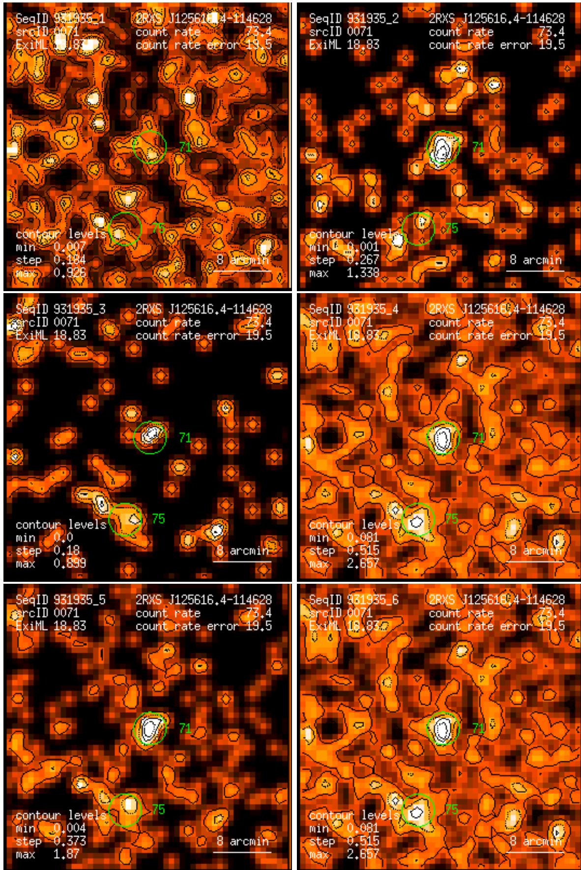
Figure 71: RASS 931935: detection 0071: band rate images, Gaussian filter: (1) PSPC channels 11 – 41, (2) 52 – 90, (3) 91 – 201, (4) 11 – 235, (5) 52 – 201, (6) 11 – 201. Broad band rates in counts/ks. Band rate contour levels in counts/ks/arcmin 2 .
