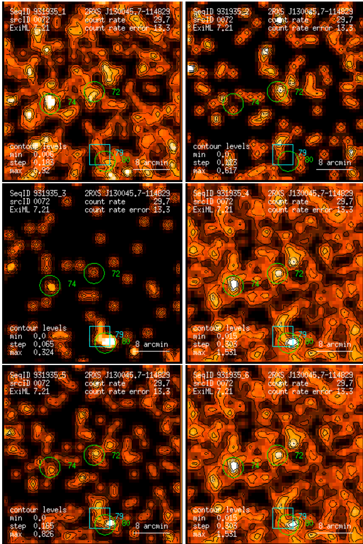
Figure 72: RASS 931935: detection 0072: band rate images, Gaussian filter: (1) PSPC channels 11 – 41, (2) 52 – 90, (3) 91 – 201, (4) 11 – 235, (5) 52 – 201, (6) 11 – 201. Broad band rates in counts/ks. Band rate contour levels in counts/ks/arcmin 2 .
