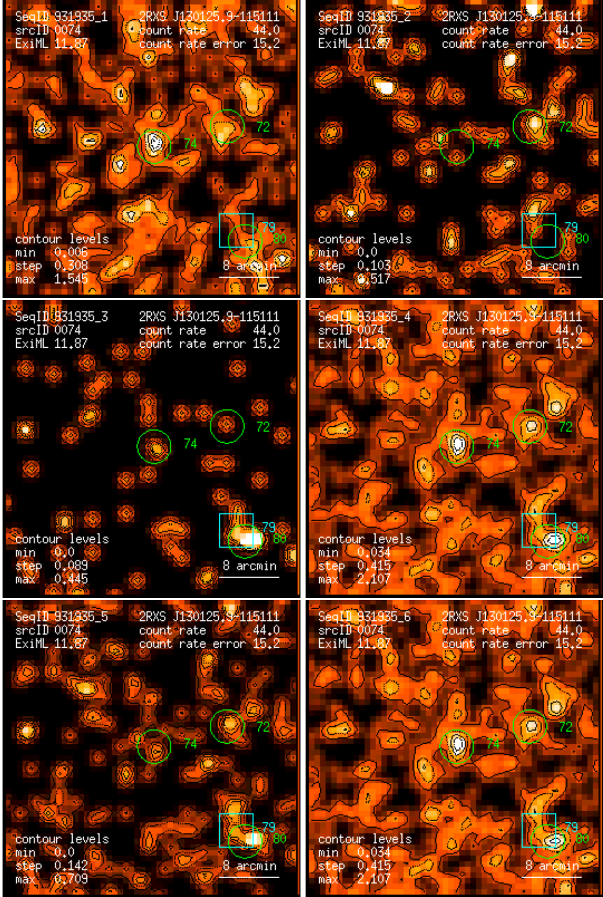
Figure 74: RASS 931935: detection 0074: band rate images, Gaussian filter: (1) PSPC channels 11 – 41, (2) 52 – 90, (3) 91 – 201, (4) 11 – 235, (5) 52 – 201, (6) 11 – 201. Broad band rates in counts/ks. Band rate contour levels in counts/ks/arcmin 2 .
