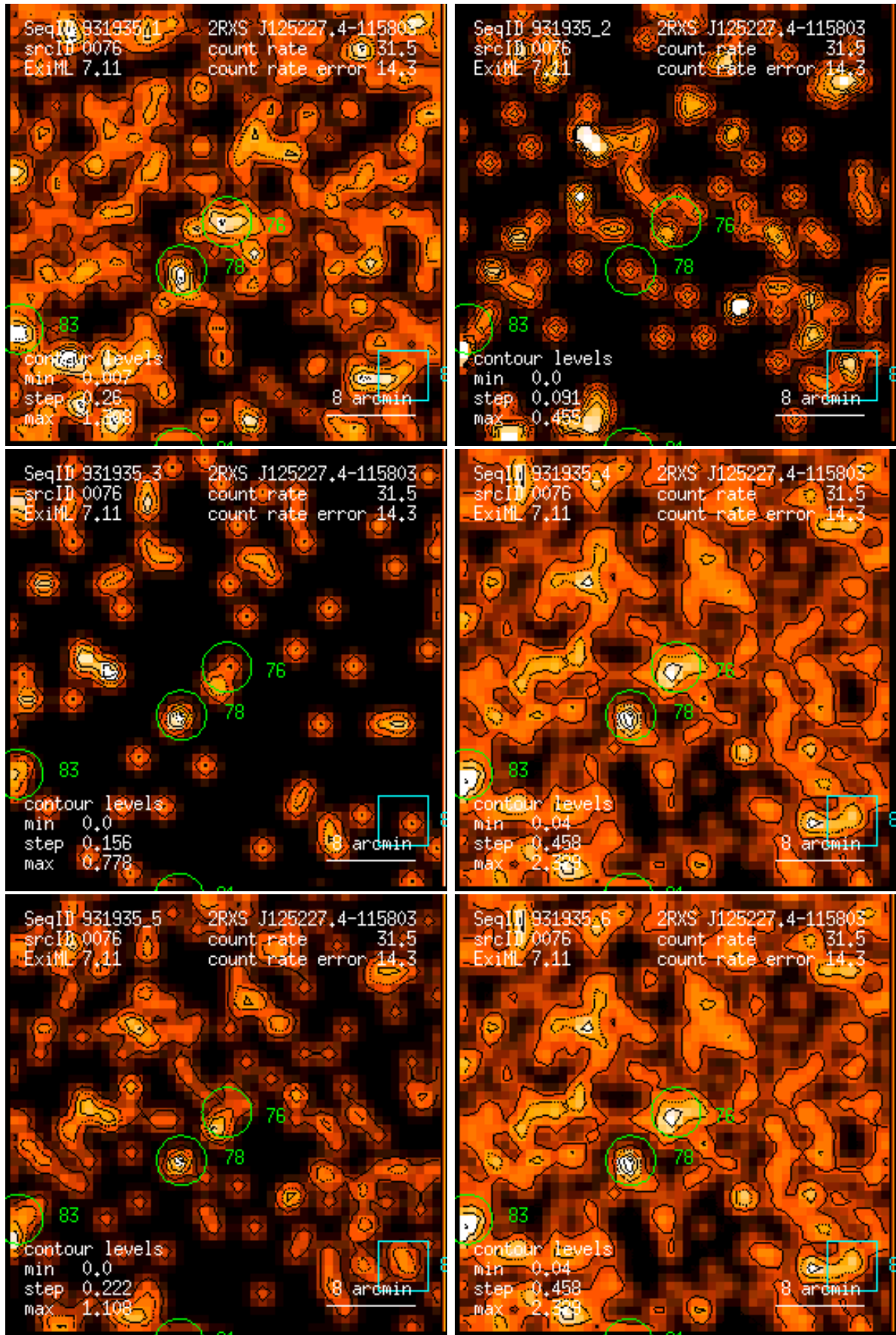
Figure 76: RASS 931935: detection 0076: band rate images, Gaussian filter: (1) PSPC channels 11 – 41, (2) 52 – 90, (3) 91 – 201, (4) 11 – 235, (5) 52 – 201, (6) 11 – 201. Broad band rates in counts/ks. Band rate contour levels in counts/ks/arcmin 2 .
