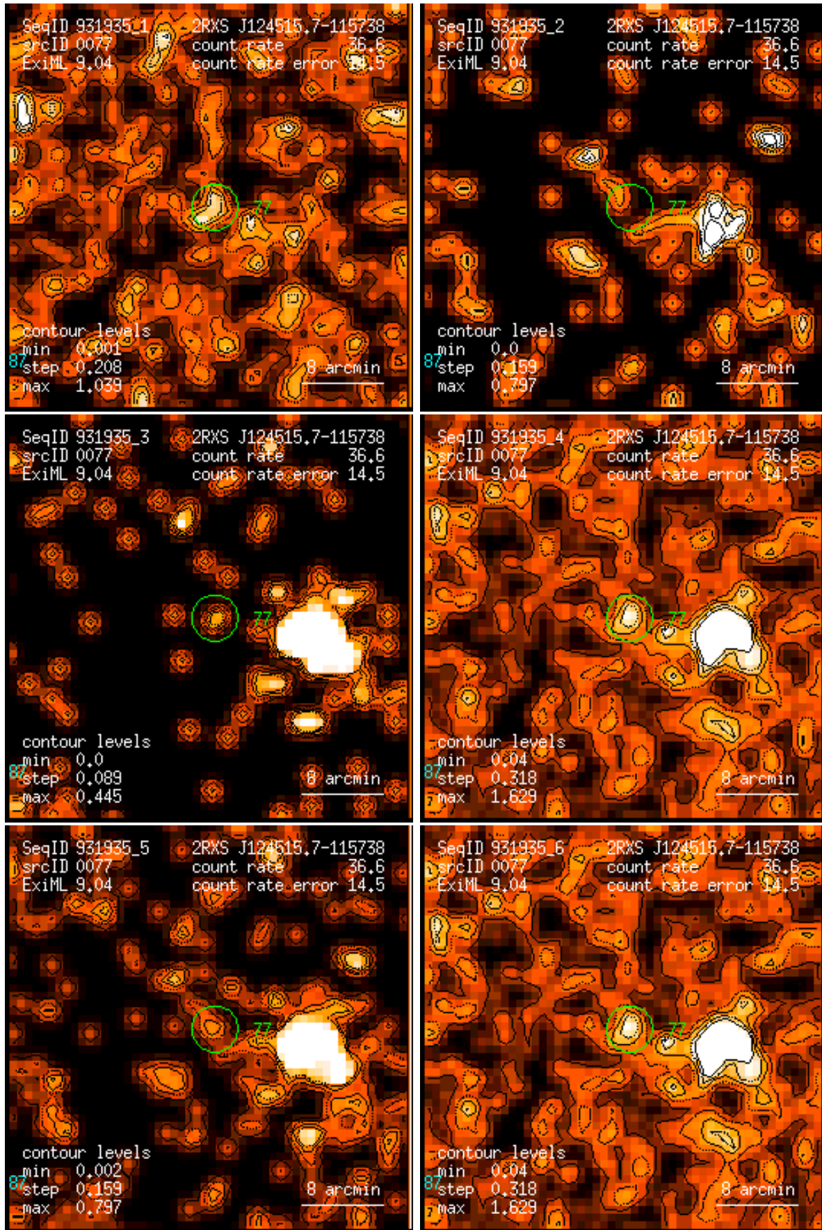
Figure 77: RASS 931935: detection 0077: band rate images, Gaussian filter: (1) PSPC channels 11 – 41, (2) 52 – 90, (3) 91 – 201, (4) 11 – 235, (5) 52 – 201, (6) 11 – 201. Broad band rates in counts/ks. Band rate contour levels in counts/ks/arcmin 2 .
