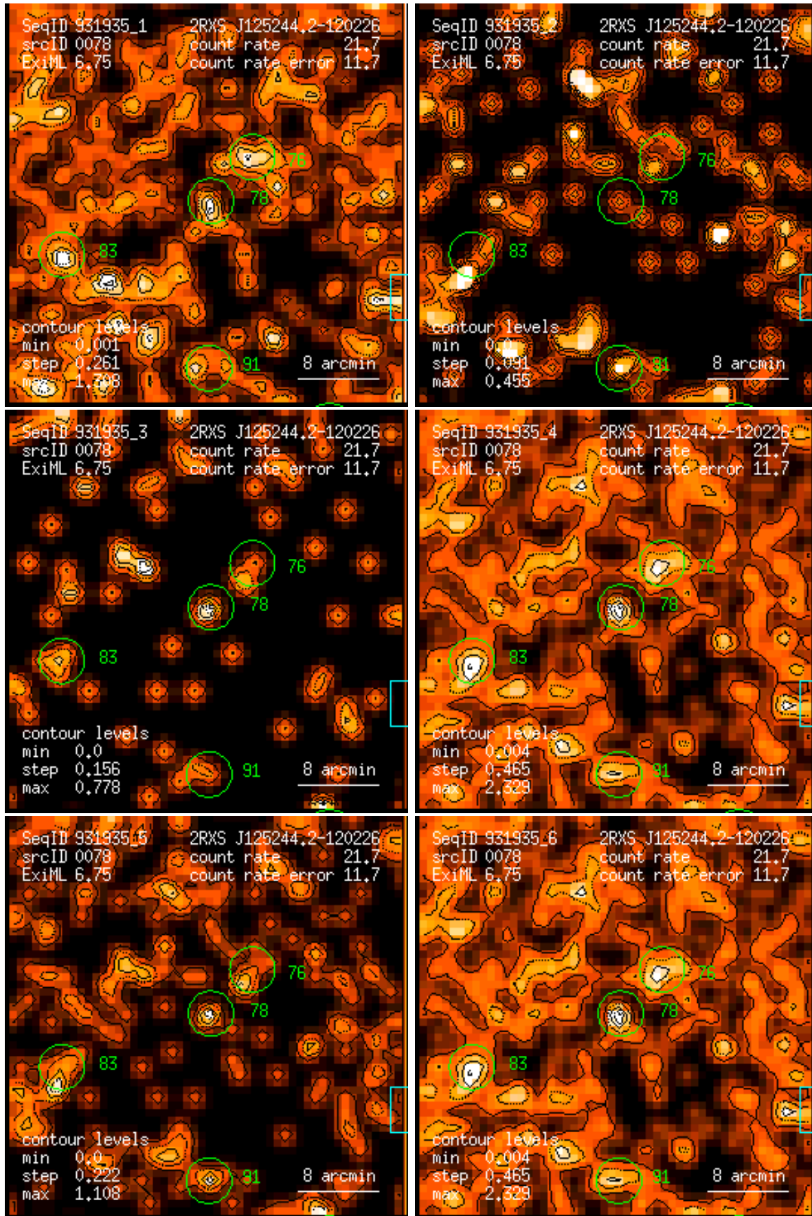
Figure 78: RASS 931935: detection 0078: band rate images, Gaussian filter: (1) PSPC channels 11 – 41, (2) 52 – 90, (3) 91 – 201, (4) 11 – 235, (5) 52 – 201, (6) 11 – 201. Broad band rates in counts/ks. Band rate contour levels in counts/ks/arcmin 2 .
