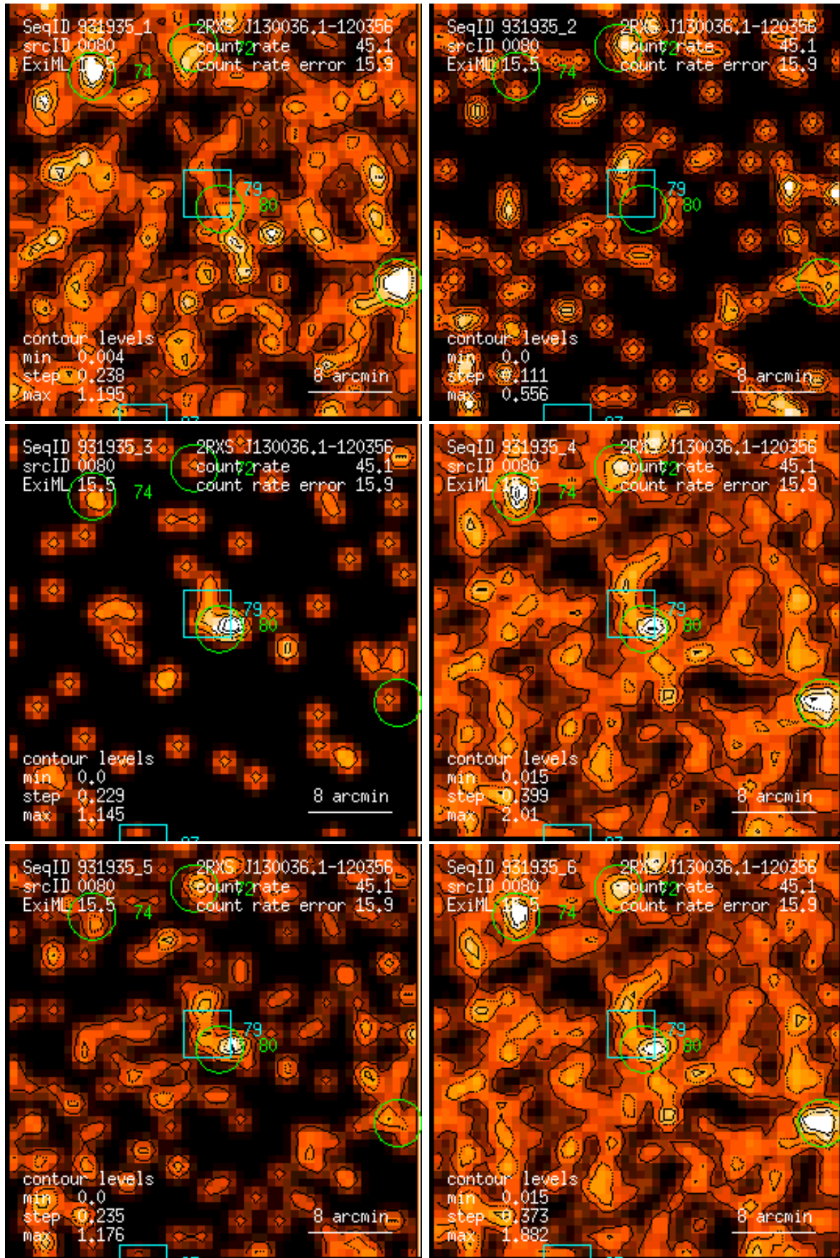
Figure 80: RASS 931935: detection 0080: band rate images, Gaussian filter: (1) PSPC channels 11 – 41, (2) 52 – 90, (3) 91 – 201, (4) 11 – 235, (5) 52 – 201, (6) 11 – 201. Broad band rates in counts/ks. Band rate contour levels in counts/ks/arcmin 2 .
