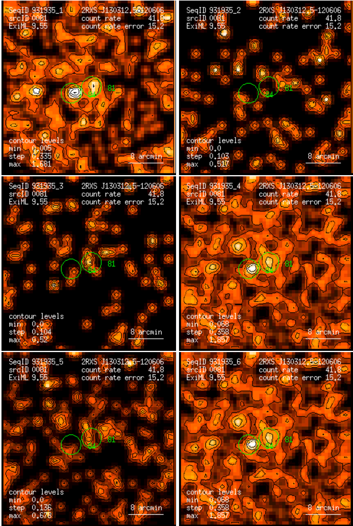
Figure 81: RASS 931935: detection 0081: band rate images, Gaussian filter: (1) PSPC channels 11 – 41, (2) 52 – 90, (3) 91 – 201, (4) 11 – 235, (5) 52 – 201, (6) 11 – 201. Broad band rates in counts/ks. Band rate contour levels in counts/ks/arcmin 2 .
