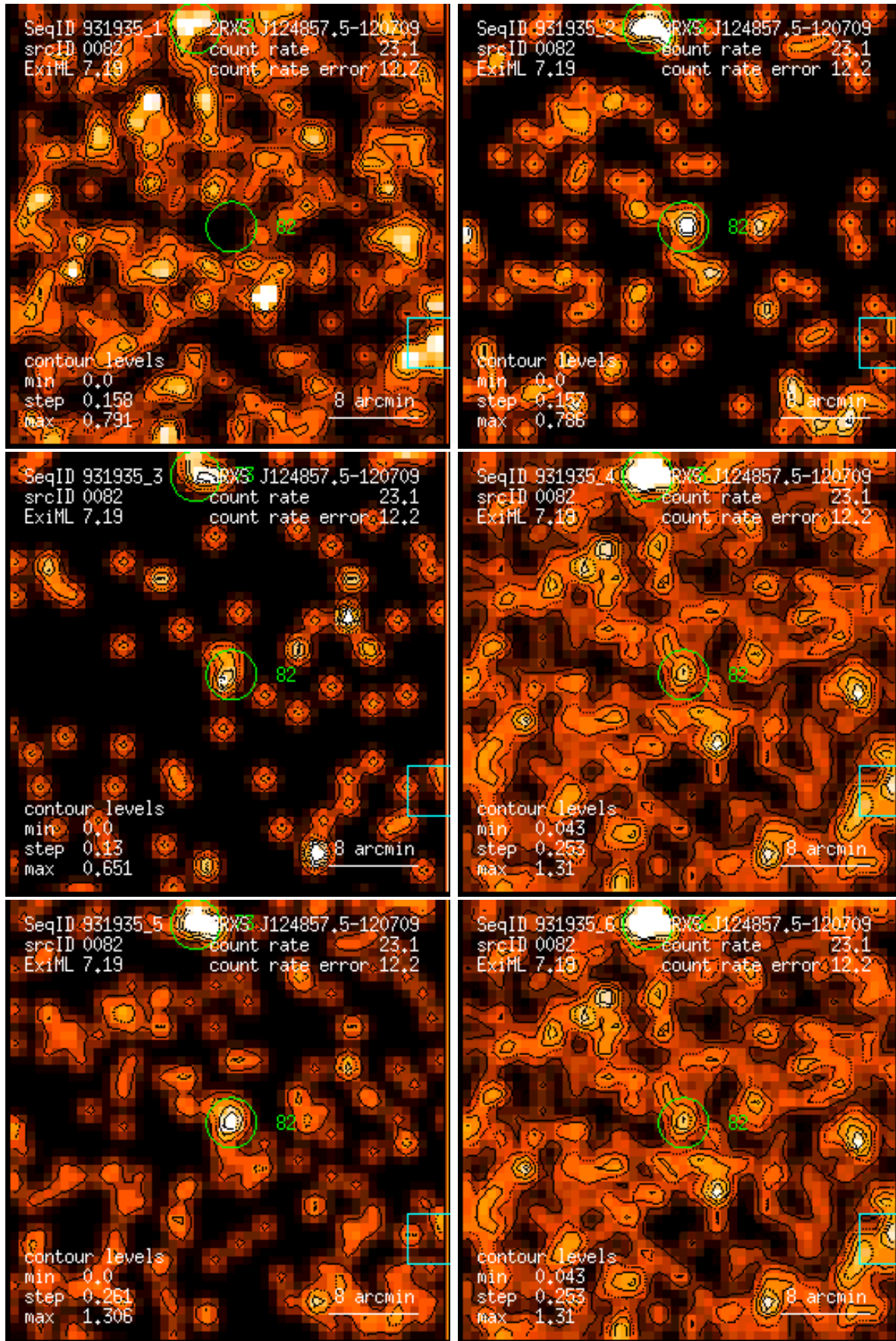
Figure 82: RASS 931935: detection 0082: band rate images, Gaussian filter: (1) PSPC channels 11 – 41, (2) 52 – 90, (3) 91 – 201, (4) 11 – 235, (5) 52 – 201, (6) 11 – 201. Broad band rates in counts/ks. Band rate contour levels in counts/ks/arcmin 2 .
