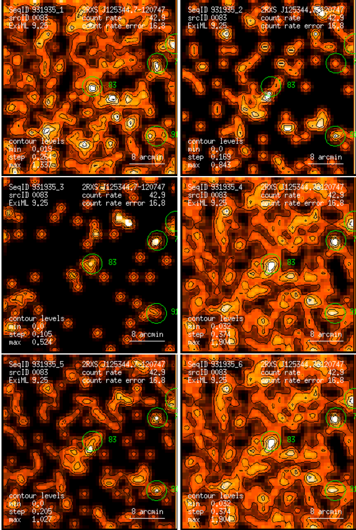
Figure 83: RASS 931935: detection 0083: band rate images, Gaussian filter: (1) PSPC channels 11 – 41, (2) 52 – 90, (3) 91 – 201, (4) 11 – 235, (5) 52 – 201, (6) 11 – 201. Broad band rates in counts/ks. Band rate contour levels in counts/ks/arcmin 2 .
