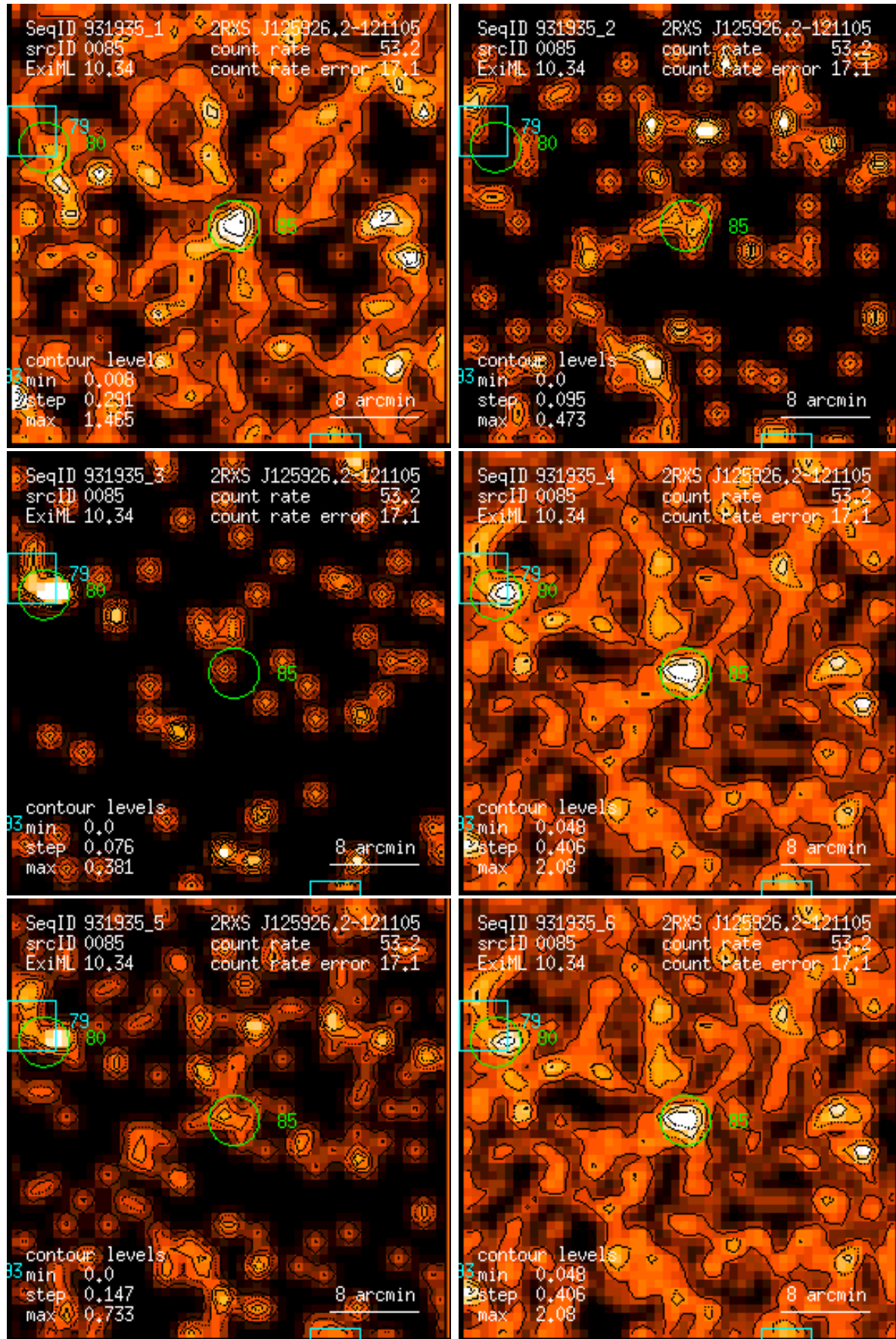
Figure 85: RASS 931935: detection 0085: band rate images, Gaussian filter: (1) PSPC channels 11 – 41, (2) 52 – 90, (3) 91 – 201, (4) 11 – 235, (5) 52 – 201, (6) 11 – 201. Broad band rates in counts/ks. Band rate contour levels in counts/ks/arcmin 2 .
