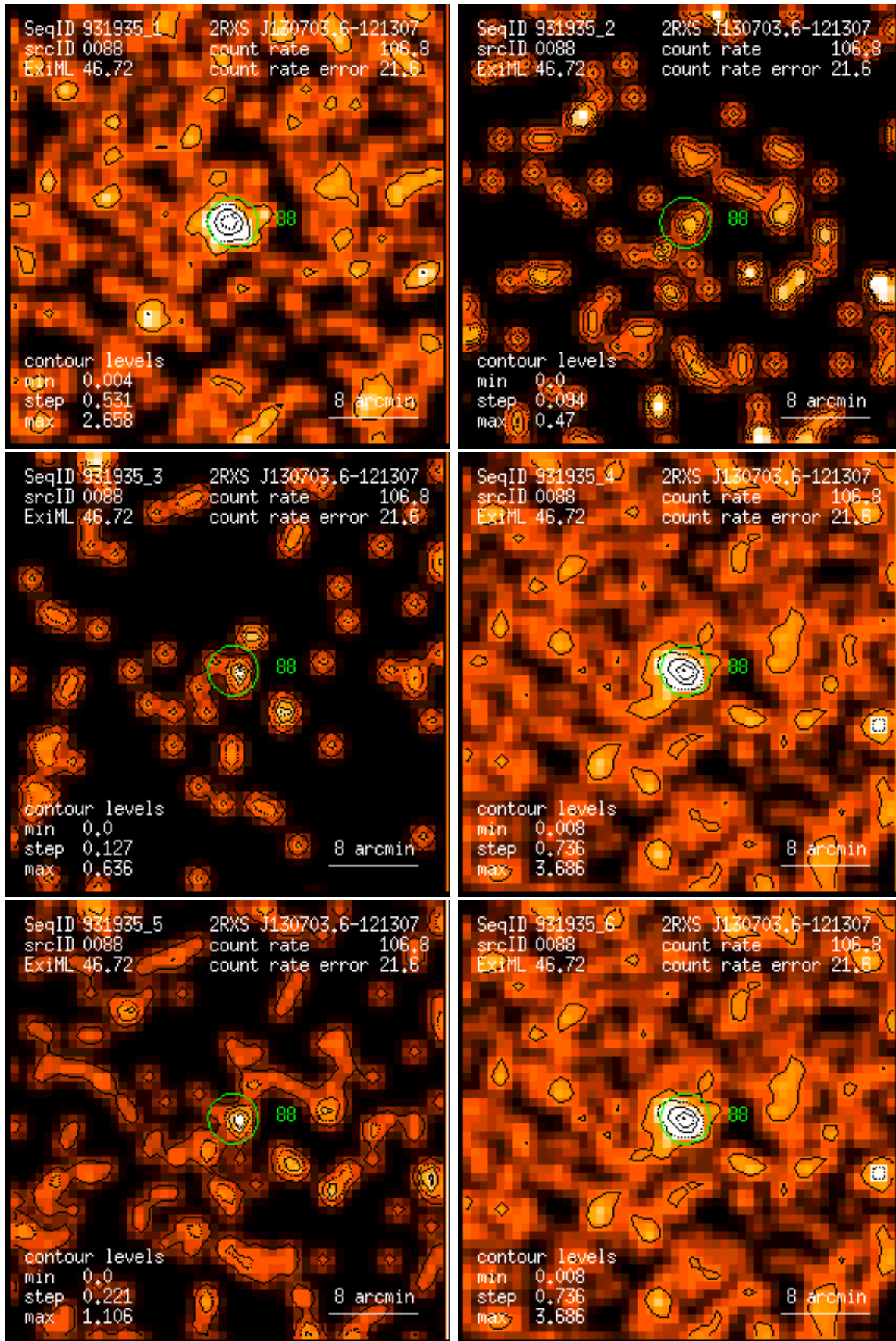
Figure 88: RASS 931935: detection 0088: band rate images, Gaussian filter: (1) PSPC channels 11 – 41, (2) 52 – 90, (3) 91 – 201, (4) 11 – 235, (5) 52 – 201, (6) 11 – 201. Broad band rates in counts/ks. Band rate contour levels in counts/ks/arcmin 2 .
