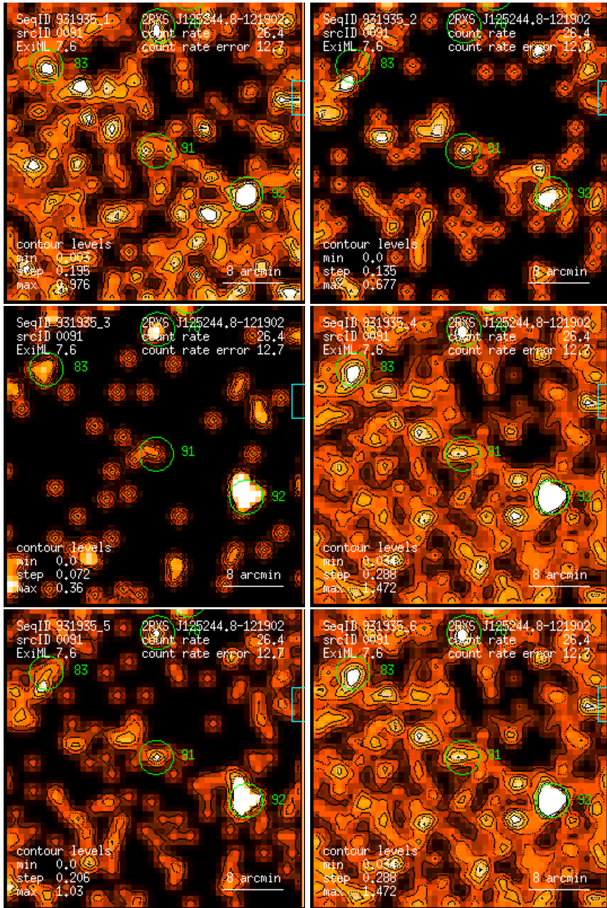
Figure 91: RASS 931935: detection 0091: band rate images, Gaussian filter: (1) PSPC channels 11 – 41, (2) 52 – 90, (3) 91 – 201, (4) 11 – 235, (5) 52 – 201, (6) 11 – 201. Broad band rates in counts/ks. Band rate contour levels in counts/ks/arcmin 2 .
