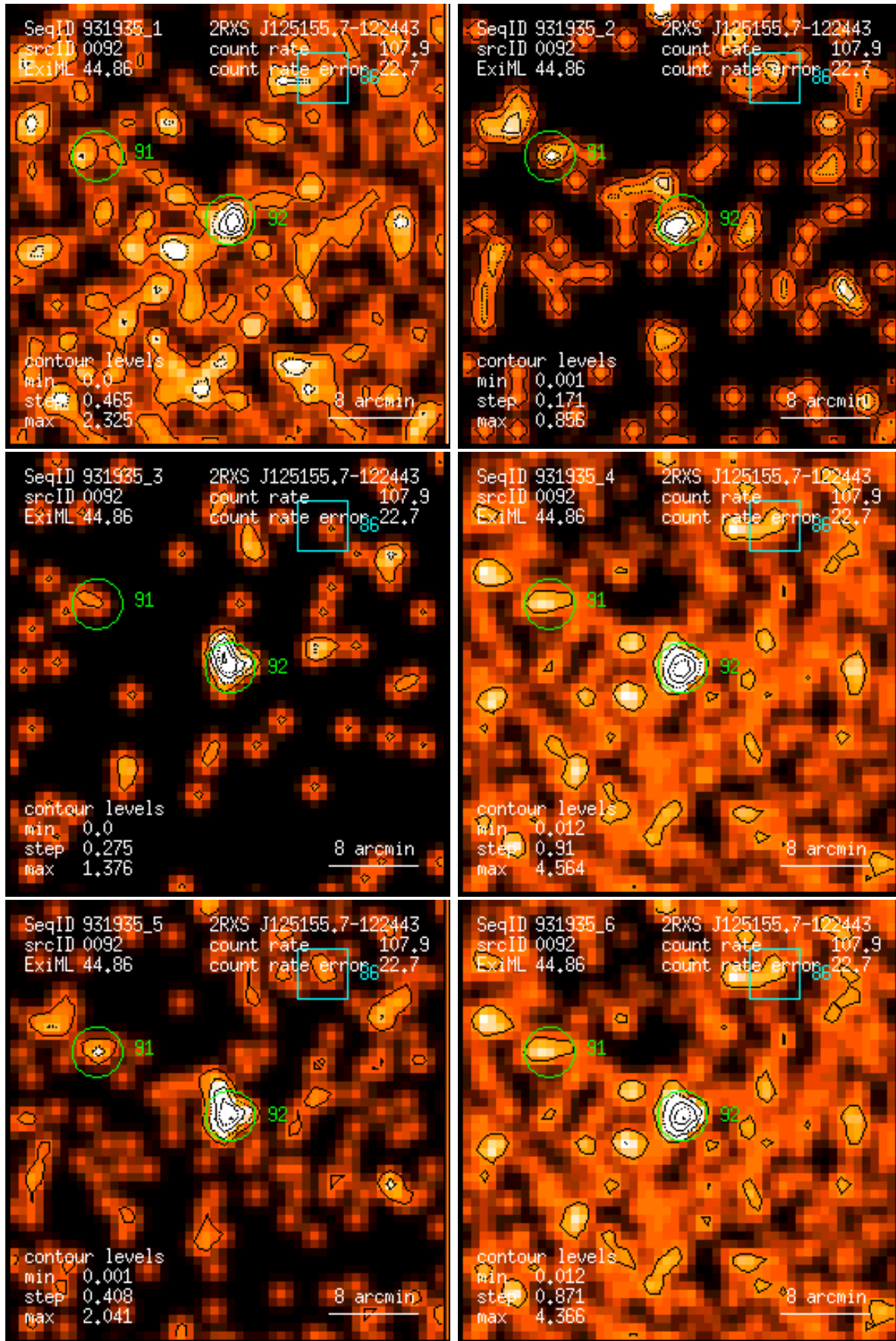
Figure 92: RASS 931935: detection 0092: band rate images, Gaussian filter: (1) PSPC channels 11 – 41, (2) 52 – 90, (3) 91 – 201, (4) 11 – 235, (5) 52 – 201, (6) 11 – 201. Broad band rates in counts/ks. Band rate contour levels in counts/ks/arcmin 2 .
