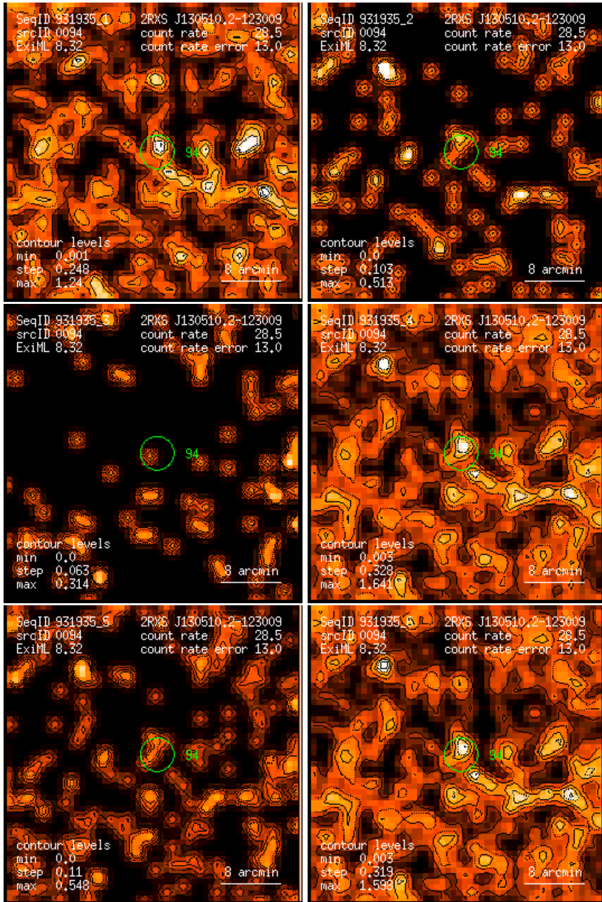
Figure 94: RASS 931935: detection 0094: band rate images, Gaussian filter: (1) PSPC channels 11 – 41, (2) 52 – 90, (3) 91 – 201, (4) 11 – 235, (5) 52 – 201, (6) 11 – 201. Broad band rates in counts/ks. Band rate contour levels in counts/ks/arcmin 2 .
