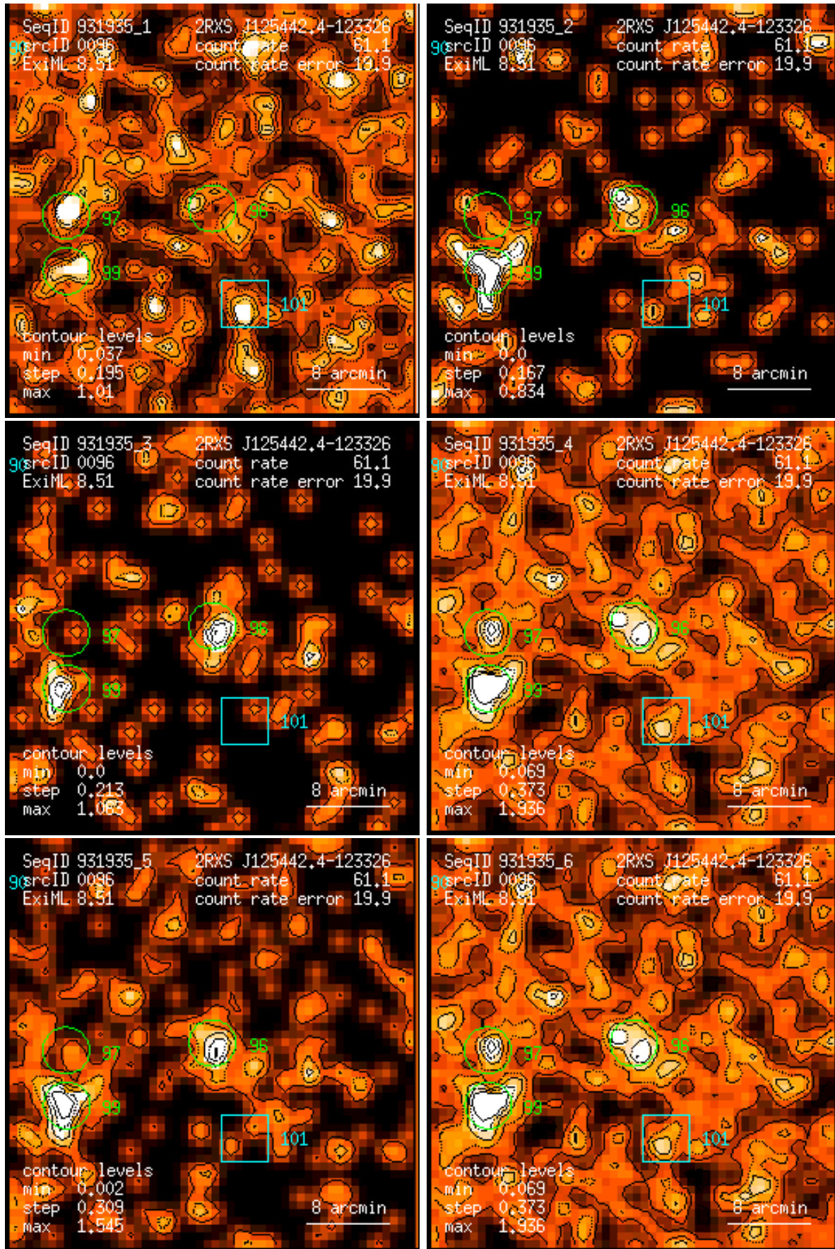
Figure 96: RASS 931935: detection 0096: band rate images, Gaussian filter: (1) PSPC channels 11 – 41, (2) 52 – 90, (3) 91 – 201, (4) 11 – 235, (5) 52 – 201, (6) 11 – 201. Broad band rates in counts/ks. Band rate contour levels in counts/ks/arcmin 2 .
