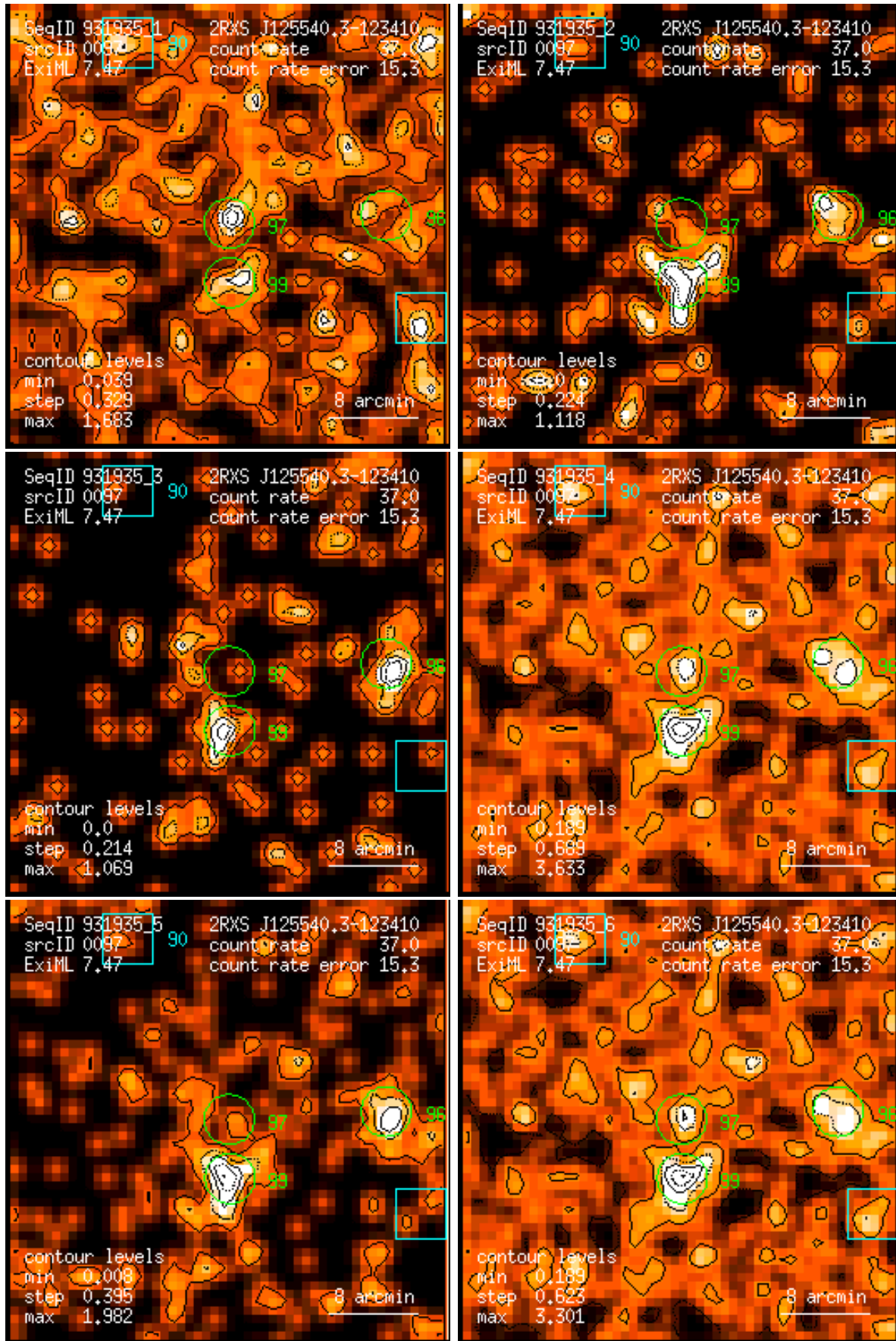
Figure 97: RASS 931935: detection 0097: band rate images, Gaussian filter: (1) PSPC channels 11 – 41, (2) 52 – 90, (3) 91 – 201, (4) 11 – 235, (5) 52 – 201, (6) 11 – 201. Broad band rates in counts/ks. Band rate contour levels in counts/ks/arcmin 2 .
