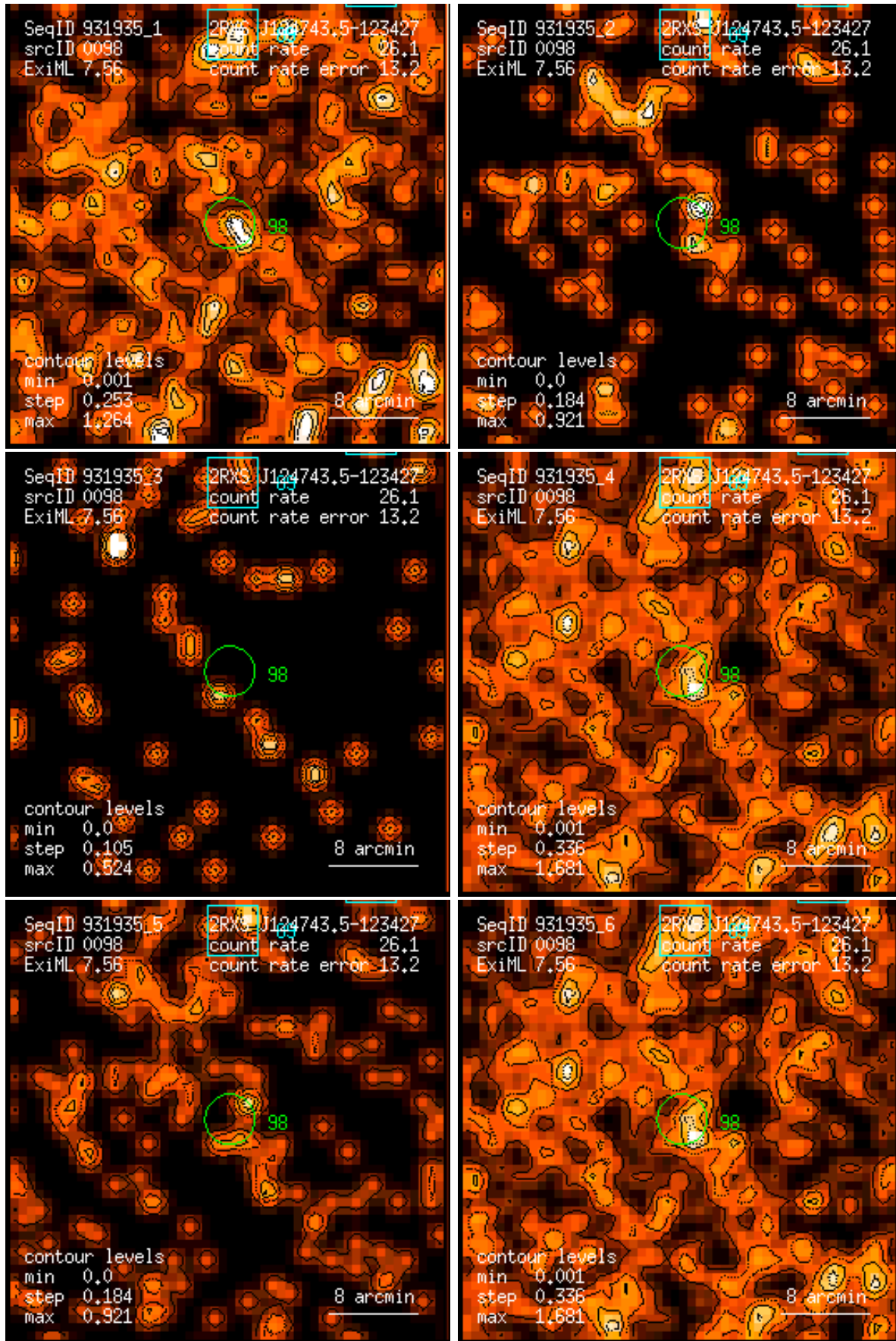
Figure 98: RASS 931935: detection 0098: band rate images, Gaussian filter: (1) PSPC channels 11 – 41, (2) 52 – 90, (3) 91 – 201, (4) 11 – 235, (5) 52 – 201, (6) 11 – 201. Broad band rates in counts/ks. Band rate contour levels in counts/ks/arcmin 2 .
