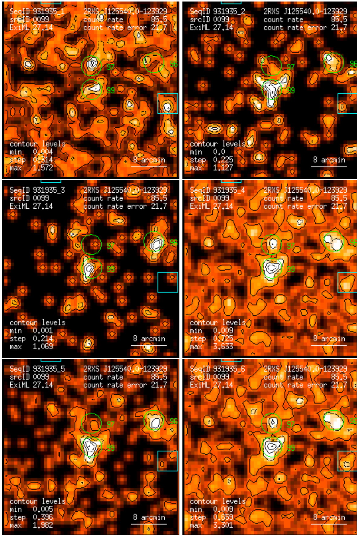
Figure 99: RASS 931935: detection 0099: band rate images, Gaussian filter: (1) PSPC channels 11 – 41, (2) 52 – 90, (3) 91 – 201, (4) 11 – 235, (5) 52 – 201, (6) 11 – 201. Broad band rates in counts/ks. Band rate contour levels in counts/ks/arcmin 2 .
