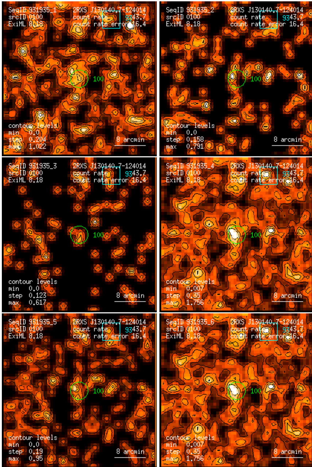
Figure 100: RASS 931935: detection 0100: band rate images, Gaussian filter: (1) PSPC channels 11 – 41, (2) 52 – 90, (3) 91 – 201, (4) 11 – 235, (5) 52 – 201, (6) 11 – 201. Broad band rates in counts/ks. Band rate contour levels in counts/ks/arcmin 2 .
