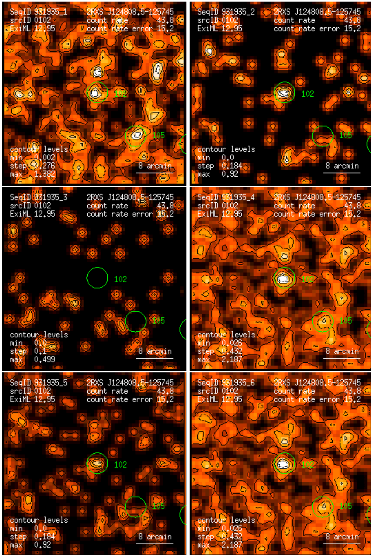
Figure 102: RASS 931935: detection 0102: band rate images, Gaussian filter: (1) PSPC channels 11 – 41, (2) 52 – 90, (3) 91 – 201, (4) 11 – 235, (5) 52 – 201, (6) 11 – 201. Broad band rates in counts/ks. Band rate contour levels in counts/ks/arcmin 2 .
