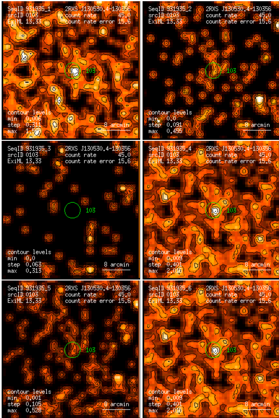
Figure 103: RASS 931935: detection 0103: band rate images, Gaussian filter: (1) PSPC channels 11 – 41, (2) 52 – 90, (3) 91 – 201, (4) 11 – 235, (5) 52 – 201, (6) 11 – 201. Broad band rates in counts/ks. Band rate contour levels in counts/ks/arcmin 2 .
